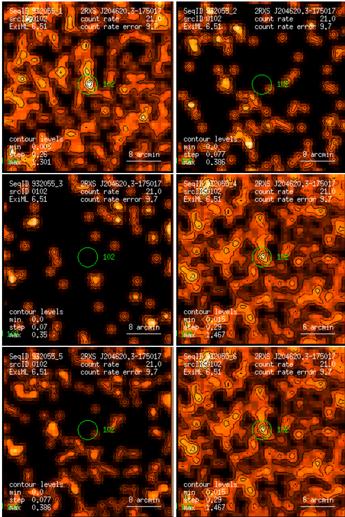
Figure 102: RASS 932055: detection 0102: band rate images, Gaussian filter: (1) PSPC channels 11 – 41, (2) 52 – 90, (3) 91 – 201, (4) 11 – 235, (5) 52 – 201, (6) 11 – 201. Broad band rates in counts/ks. Band rate contour levels in counts/ks/arcmin 2 .
