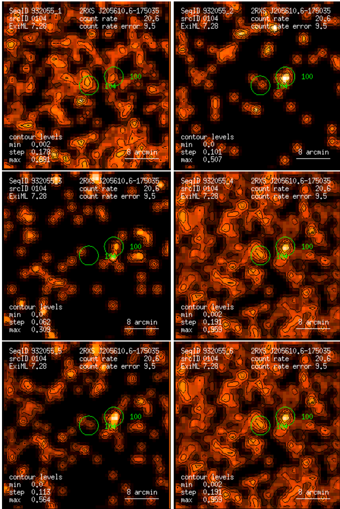
Figure 104: RASS 932055: detection 0104: band rate images, Gaussian filter: (1) PSPC channels 11 – 41, (2) 52 – 90, (3) 91 – 201, (4) 11 – 235, (5) 52 – 201, (6) 11 – 201. Broad band rates in counts/ks. Band rate contour levels in counts/ks/arcmin 2 .
