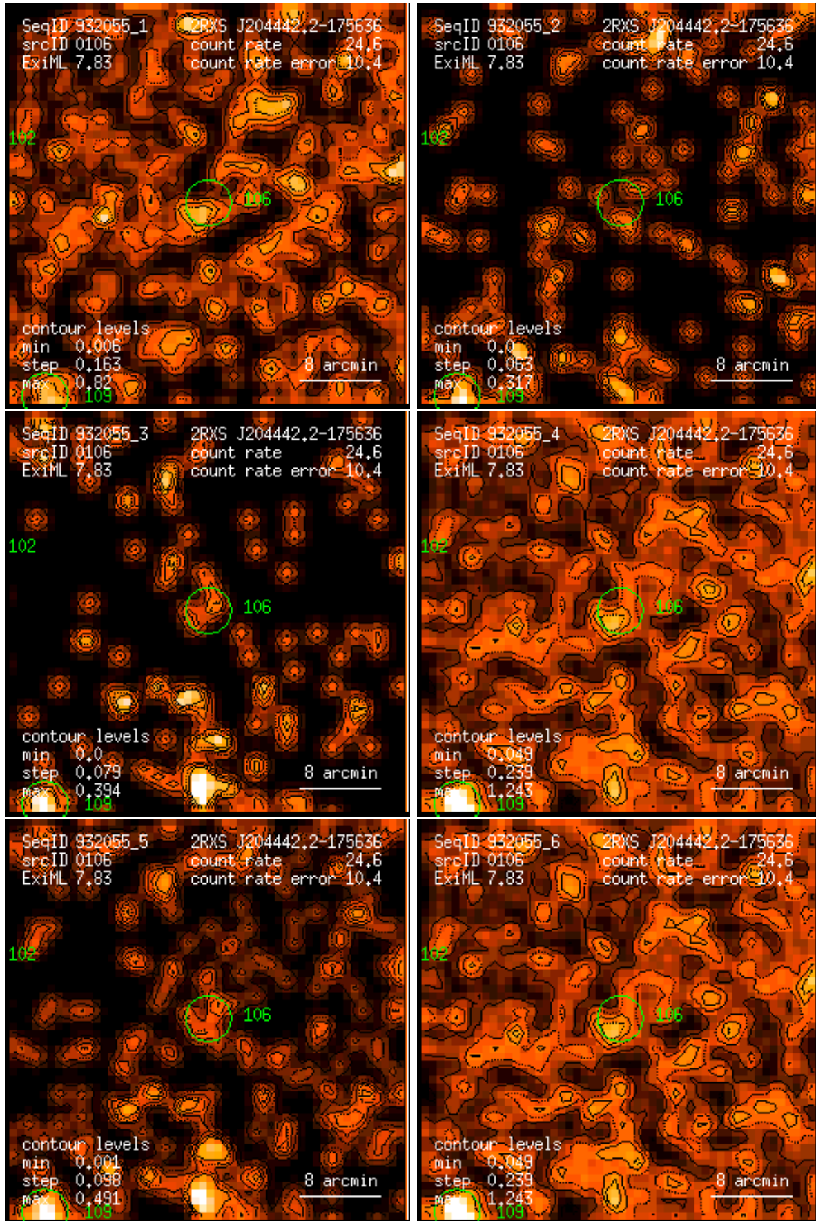
Figure 106: RASS 932055: detection 0106: band rate images, Gaussian filter: (1) PSPC channels 11 – 41, (2) 52 – 90, (3) 91 – 201, (4) 11 – 235, (5) 52 – 201, (6) 11 – 201. Broad band rates in counts/ks. Band rate contour levels in counts/ks/arcmin 2 .
