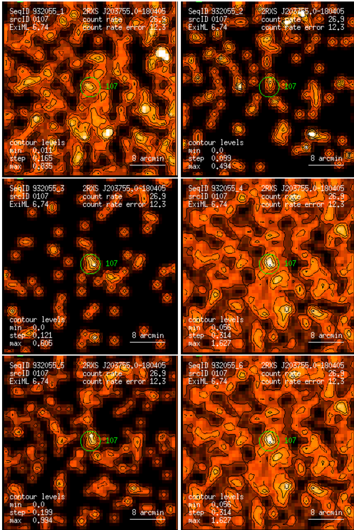
Figure 107: RASS 932055: detection 0107: band rate images, Gaussian filter: (1) PSPC channels 11 – 41, (2) 52 – 90, (3) 91 – 201, (4) 11 – 235, (5) 52 – 201, (6) 11 – 201. Broad band rates in counts/ks. Band rate contour levels in counts/ks/arcmin 2 .
