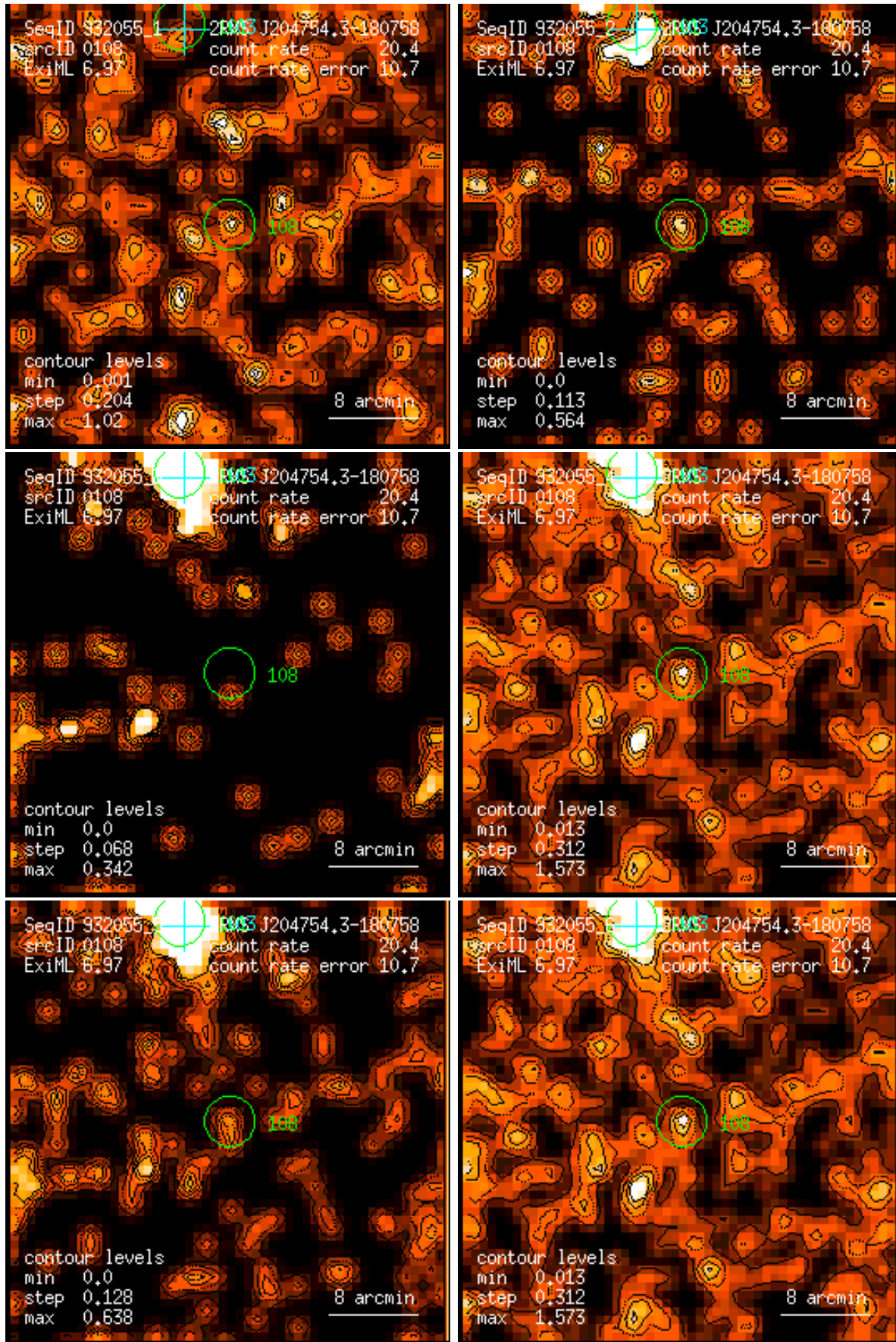
Figure 108: RASS 932055: detection 0108: band rate images, Gaussian filter: (1) PSPC channels 11 – 41, (2) 52 – 90, (3) 91 – 201, (4) 11 – 235, (5) 52 – 201, (6) 11 – 201. Broad band rates in counts/ks. Band rate contour levels in counts/ks/arcmin 2 .
