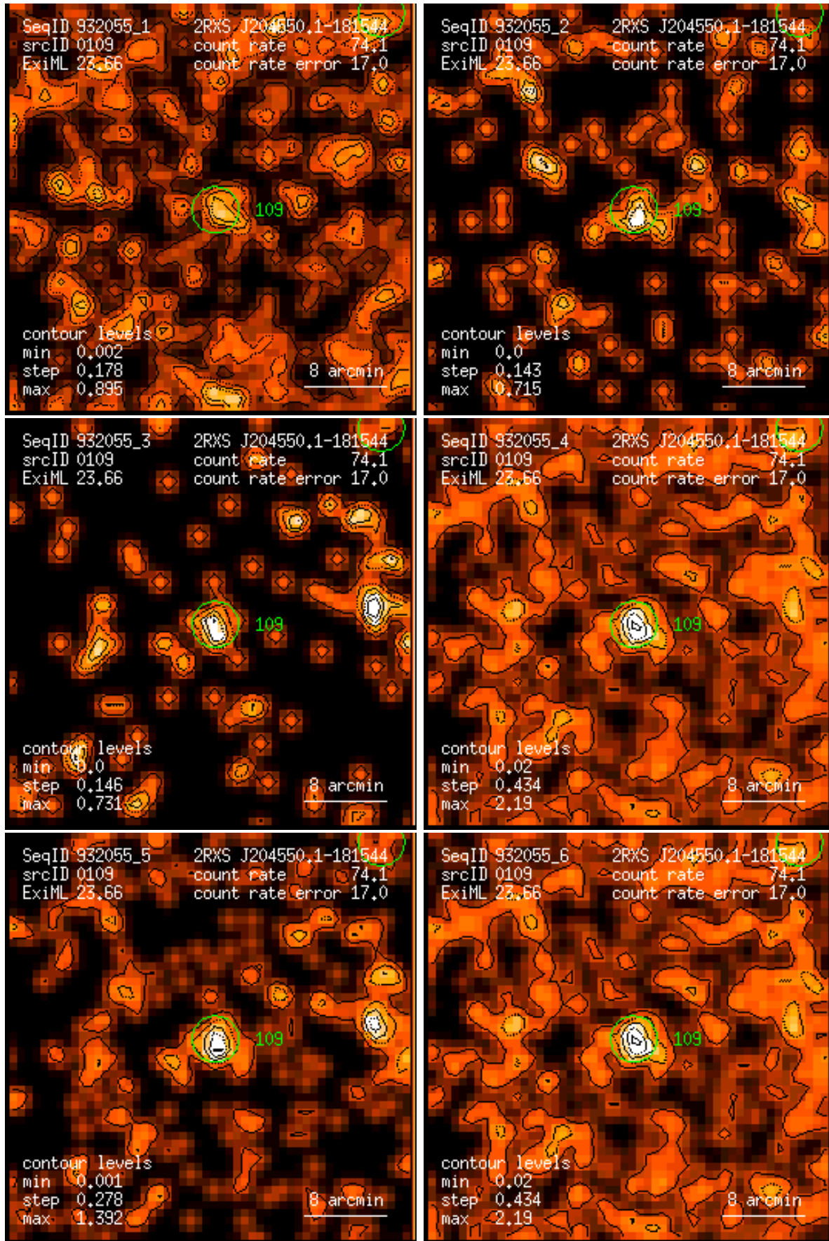
Figure 109: RASS 932055: detection 0109: band rate images, Gaussian filter: (1) PSPC channels 11 – 41, (2) 52 – 90, (3) 91 – 201, (4) 11 – 235, (5) 52 – 201, (6) 11 – 201. Broad band rates in counts/ks. Band rate contour levels in counts/ks/arcmin 2 .
