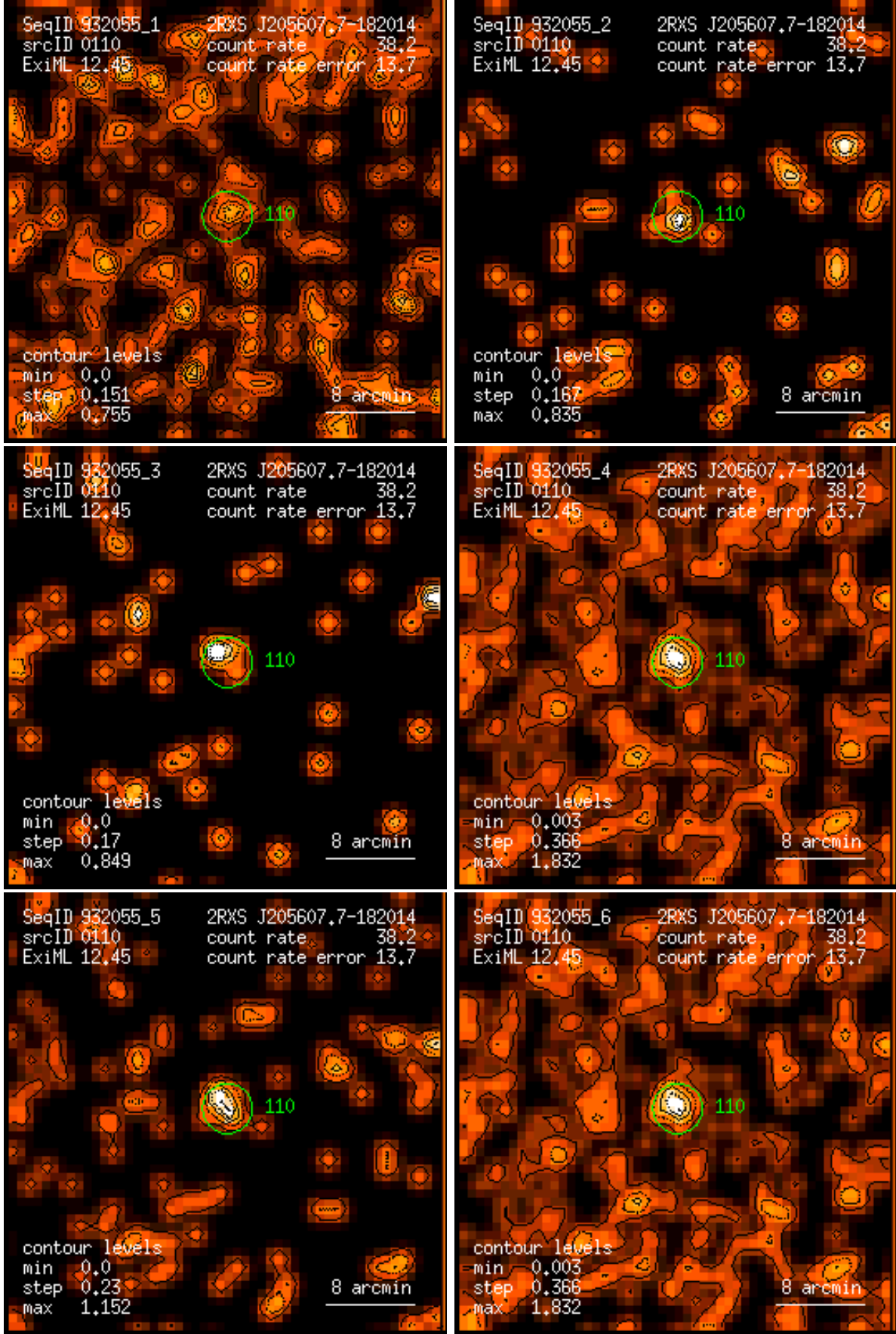
Figure 110: RASS 932055: detection 0110: band rate images, Gaussian filter: (1) PSPC channels 11 – 41, (2) 52 – 90, (3) 91 – 201, (4) 11 – 235, (5) 52 – 201, (6) 11 – 201. Broad band rates in counts/ks. Band rate contour levels in counts/ks/arcmin 2 .
