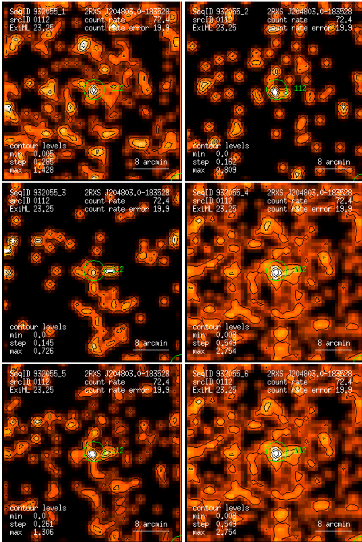
Figure 112: RASS 932055: detection 0112: band rate images, Gaussian filter: (1) PSPC channels 11 – 41, (2) 52 – 90, (3) 91 – 201, (4) 11 – 235, (5) 52 – 201, (6) 11 – 201. Broad band rates in counts/ks. Band rate contour levels in counts/ks/arcmin 2 .
