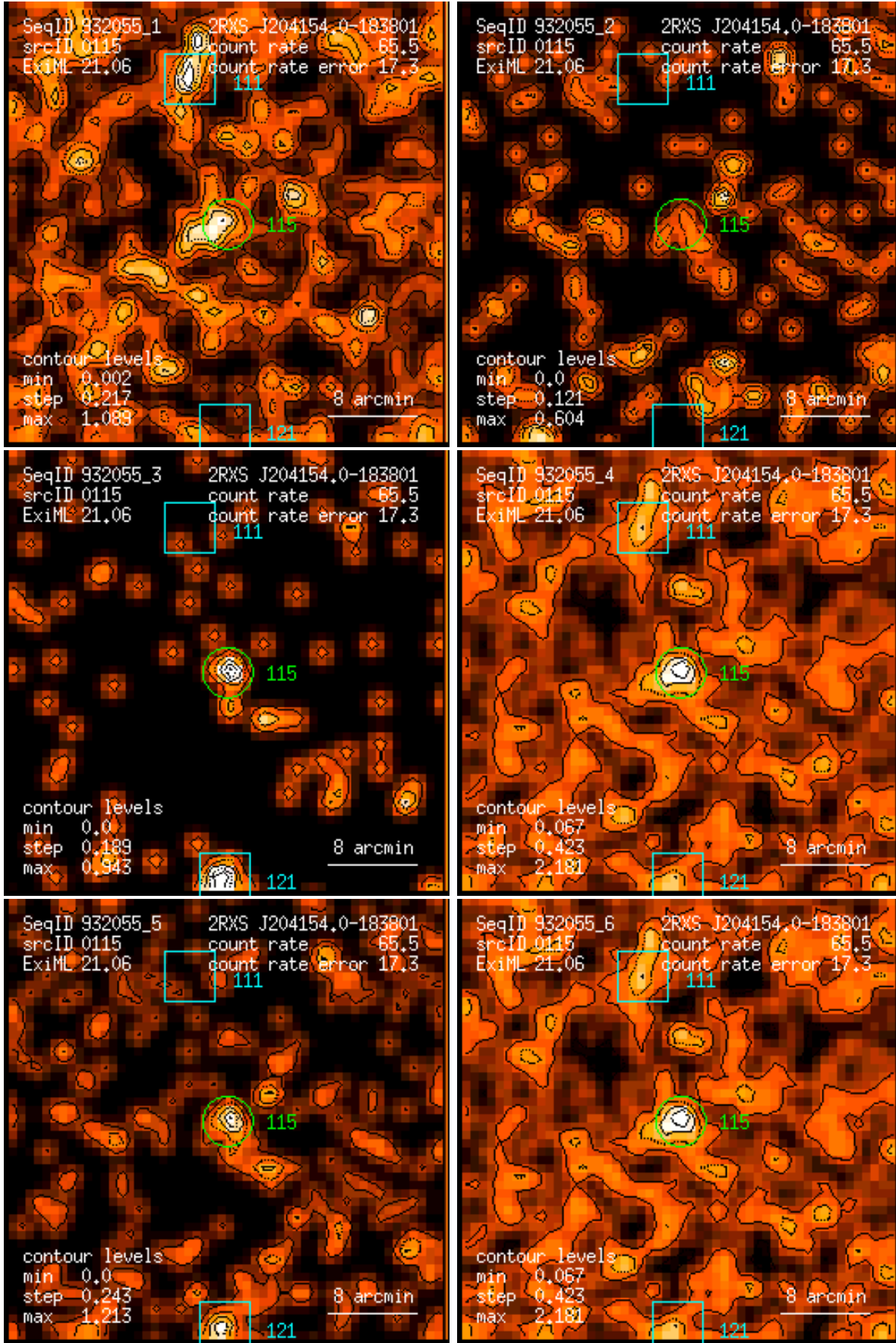
Figure 115: RASS 932055: detection 0115: band rate images, Gaussian filter: (1) PSPC channels 11 – 41, (2) 52 – 90, (3) 91 – 201, (4) 11 – 235, (5) 52 – 201, (6) 11 – 201. Broad band rates in counts/ks. Band rate contour levels in counts/ks/arcmin 2 .
