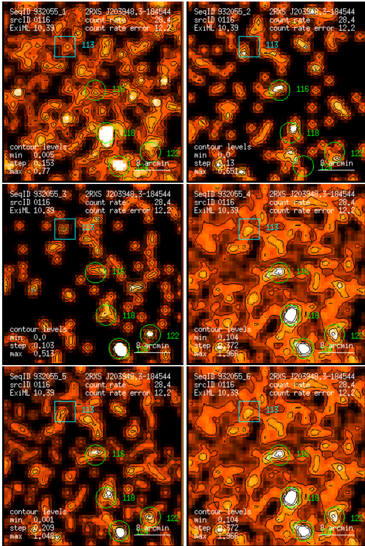
Figure 116: RASS 932055: detection 0116: band rate images, Gaussian filter: (1) PSPC channels 11 – 41, (2) 52 – 90, (3) 91 – 201, (4) 11 – 235, (5) 52 – 201, (6) 11 – 201. Broad band rates in counts/ks. Band rate contour levels in counts/ks/arcmin 2 .
