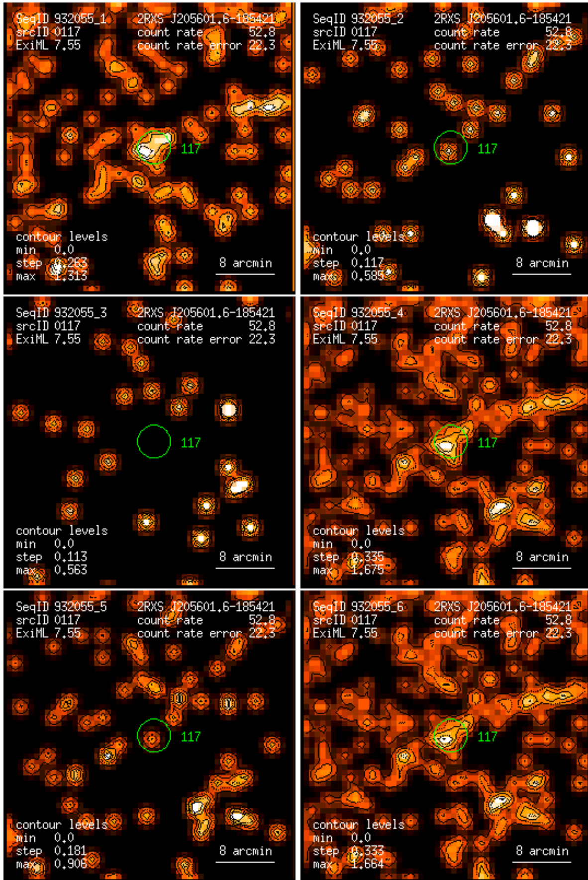
Figure 117: RASS 932055: detection 0117: band rate images, Gaussian filter: (1) PSPC channels 11 – 41, (2) 52 – 90, (3) 91 – 201, (4) 11 – 235, (5) 52 – 201, (6) 11 – 201. Broad band rates in counts/ks. Band rate contour levels in counts/ks/arcmin 2 .
