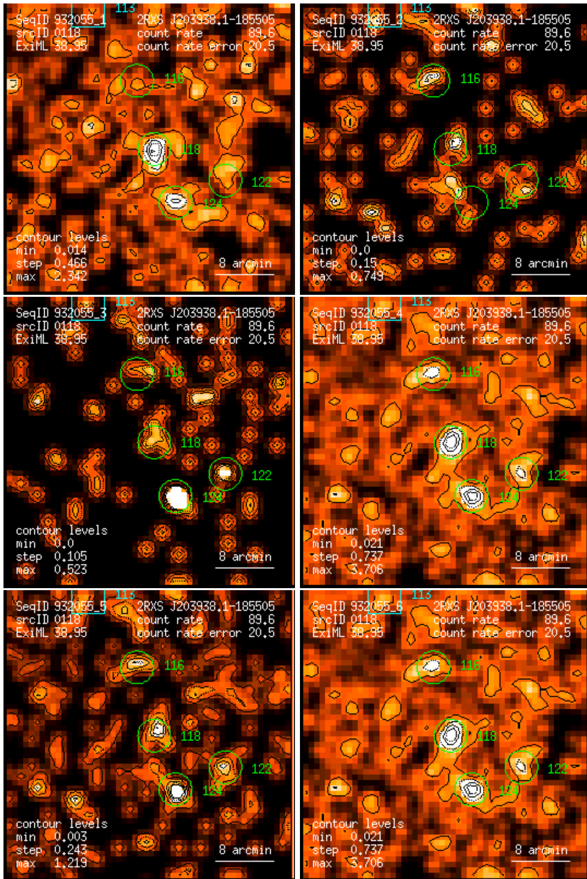
Figure 118: RASS 932055: detection 0118: band rate images, Gaussian filter: (1) PSPC channels 11 – 41, (2) 52 – 90, (3) 91 – 201, (4) 11 – 235, (5) 52 – 201, (6) 11 – 201. Broad band rates in counts/ks. Band rate contour levels in counts/ks/arcmin 2 .
