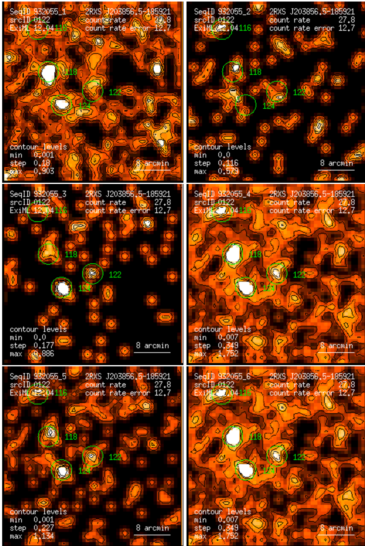
Figure 122: RASS 932055: detection 0122: band rate images, Gaussian filter: (1) PSPC channels 11 – 41, (2) 52 – 90, (3) 91 – 201, (4) 11 – 235, (5) 52 – 201, (6) 11 – 201. Broad band rates in counts/ks. Band rate contour levels in counts/ks/arcmin 2 .
