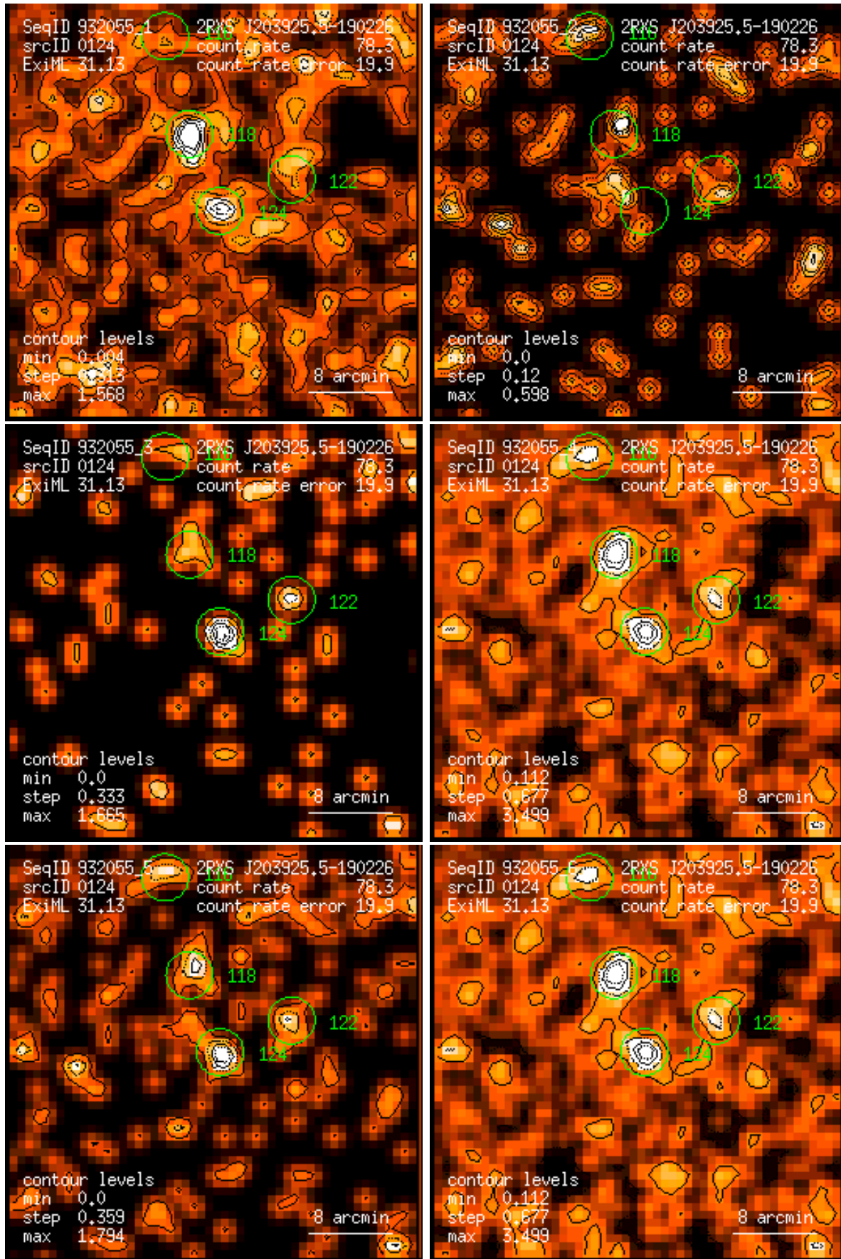
Figure 124: RASS 932055: detection 0124: band rate images, Gaussian filter: (1) PSPC channels 11 – 41, (2) 52 – 90, (3) 91 – 201, (4) 11 – 235, (5) 52 – 201, (6) 11 – 201. Broad band rates in counts/ks. Band rate contour levels in counts/ks/arcmin 2 .
