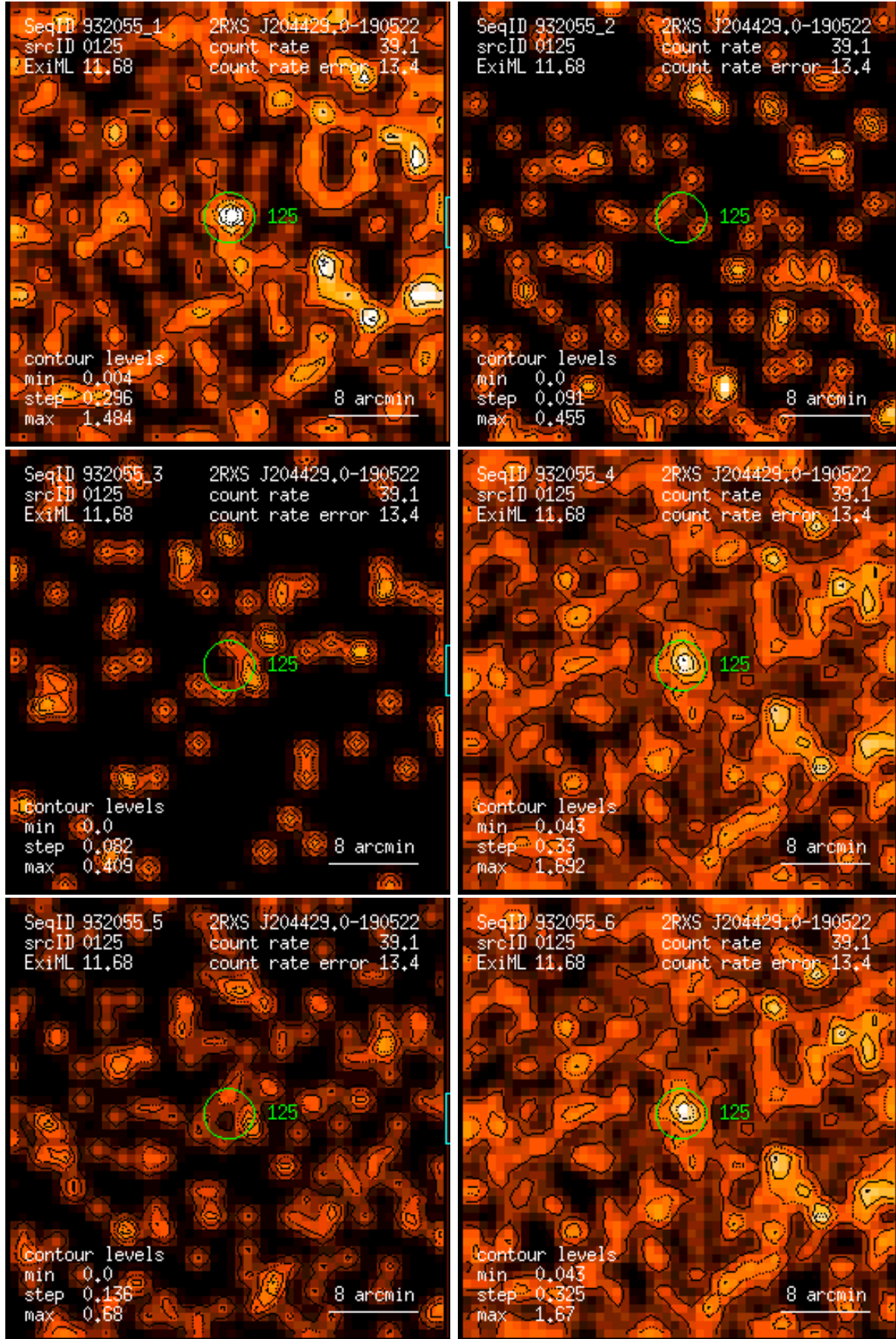
Figure 125: RASS 932055: detection 0125: band rate images, Gaussian filter: (1) PSPC channels 11 – 41, (2) 52 – 90, (3) 91 – 201, (4) 11 – 235, (5) 52 – 201, (6) 11 – 201. Broad band rates in counts/ks. Band rate contour levels in counts/ks/arcmin 2 .
