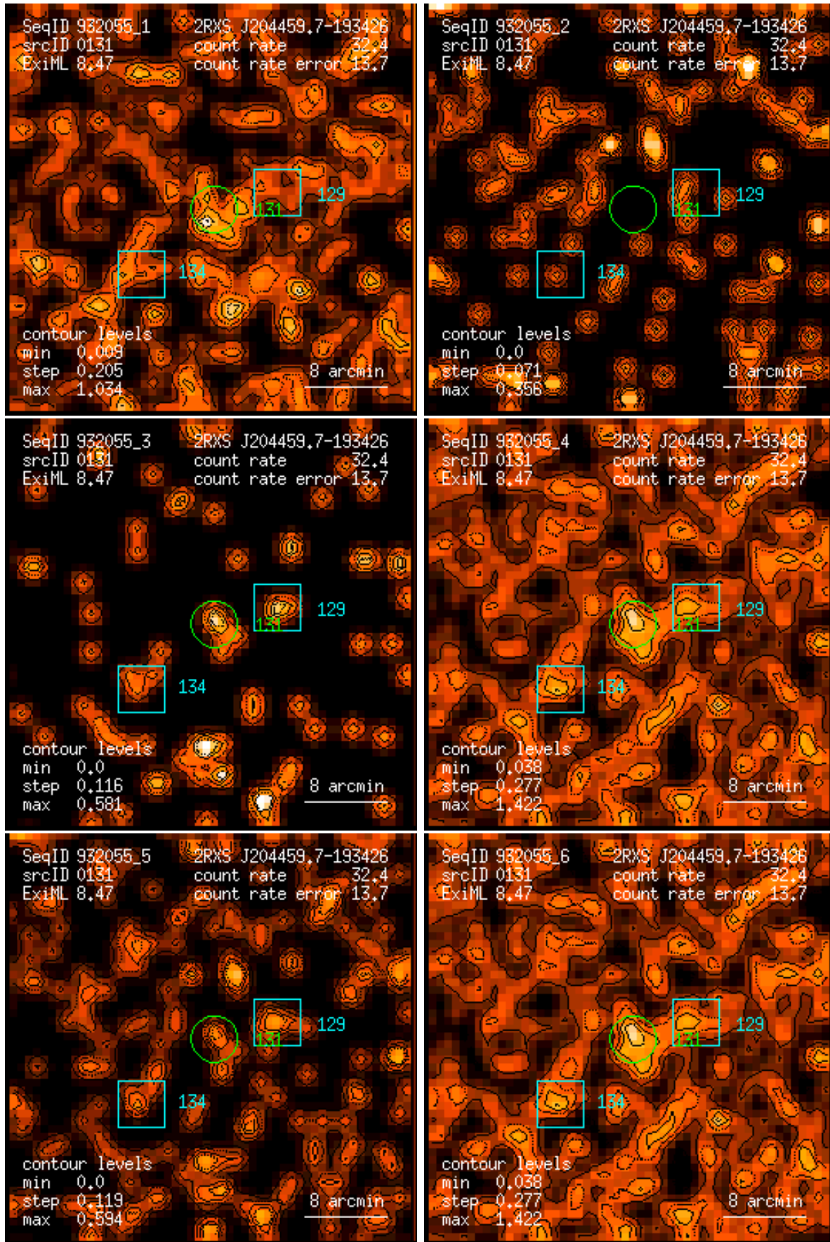
Figure 131: RASS 932055: detection 0131: band rate images, Gaussian filter: (1) PSPC channels 11 – 41, (2) 52 – 90, (3) 91 – 201, (4) 11 – 235, (5) 52 – 201, (6) 11 – 201. Broad band rates in counts/ks. Band rate contour levels in counts/ks/arcmin 2 .
