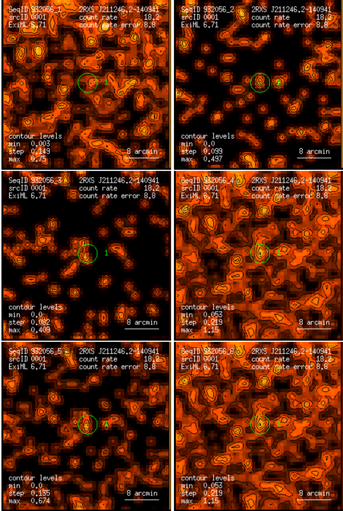
Figure 1: RASS 932056: detection 0001: band rate images, Gaussian filter: (1) PSPC channels 11 – 41, (2) 52 – 90, (3) 91 – 201, (4) 11 – 235, (5) 52 – 201, (6) 11 – 201. Broad band rates in counts/ks. Band rate contour levels in counts/ks/arcmin 2 .
