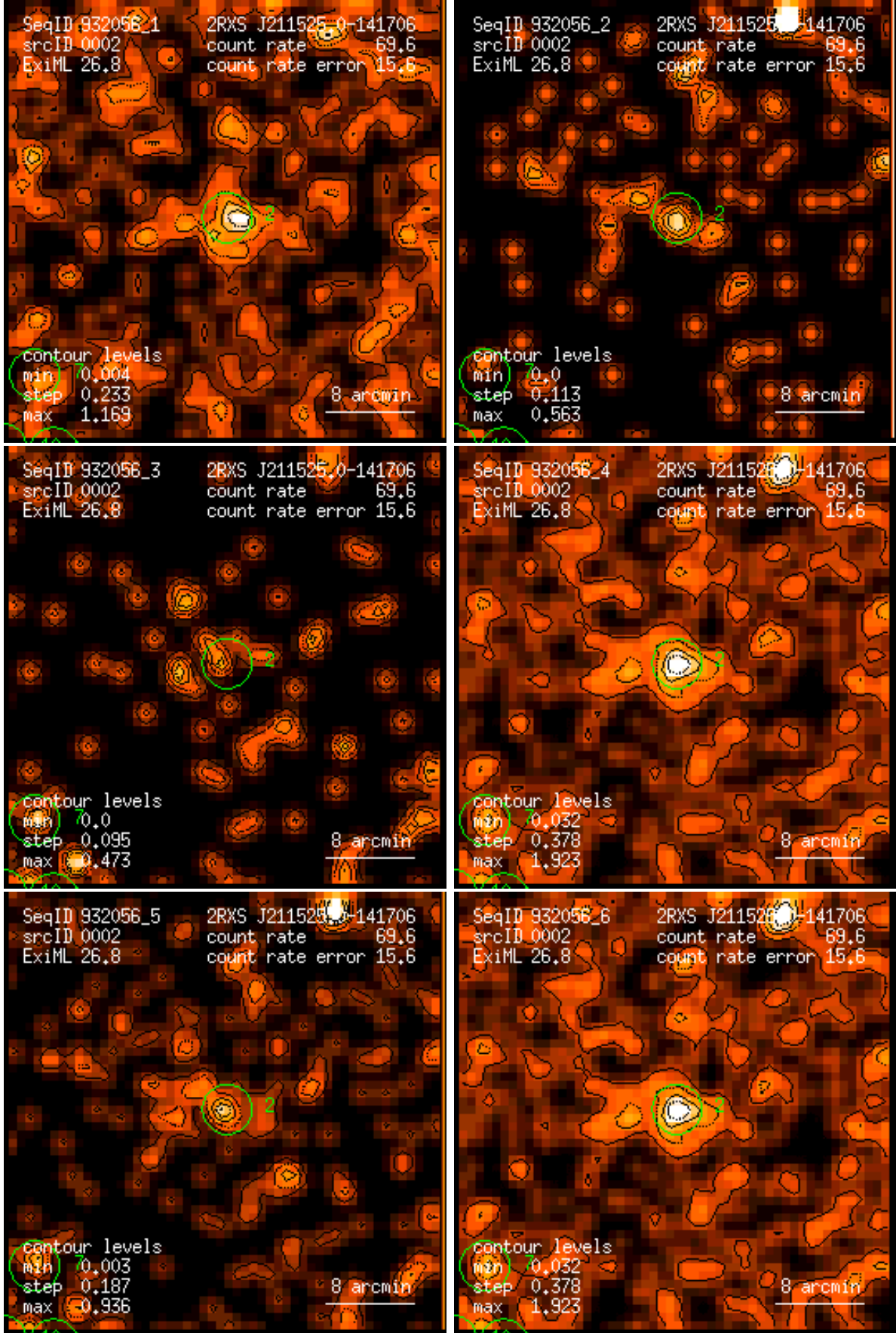
Figure 2: RASS 932056: detection 0002: band rate images, Gaussian filter: (1) PSPC channels 11 – 41, (2) 52 – 90, (3) 91 – 201, (4) 11 – 235, (5) 52 – 201, (6) 11 – 201. Broad band rates in counts/ks. Band rate contour levels in counts/ks/arcmin 2 .
