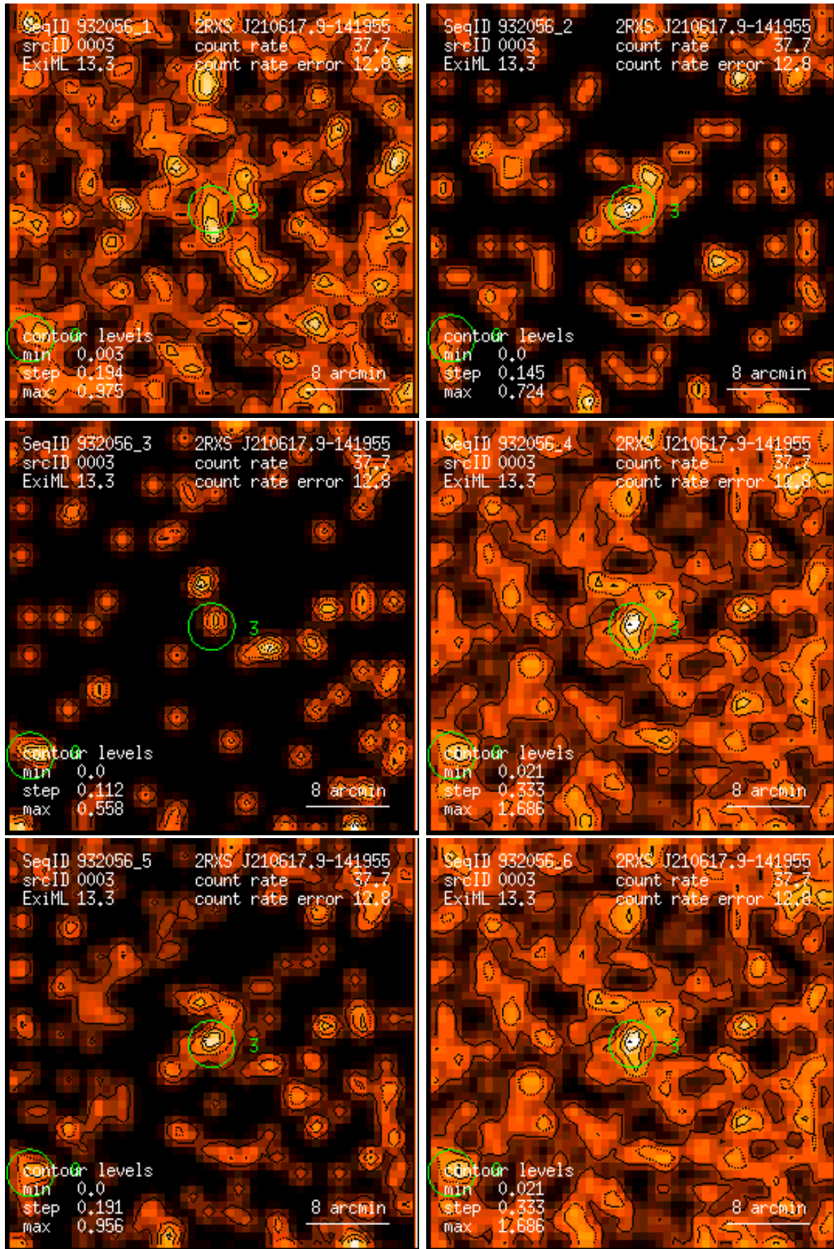
Figure 3: RASS 932056: detection 0003: band rate images, Gaussian filter: (1) PSPC channels 11 – 41, (2) 52 – 90, (3) 91 – 201, (4) 11 – 235, (5) 52 – 201, (6) 11 – 201. Broad band rates in counts/ks. Band rate contour levels in counts/ks/arcmin 2 .
