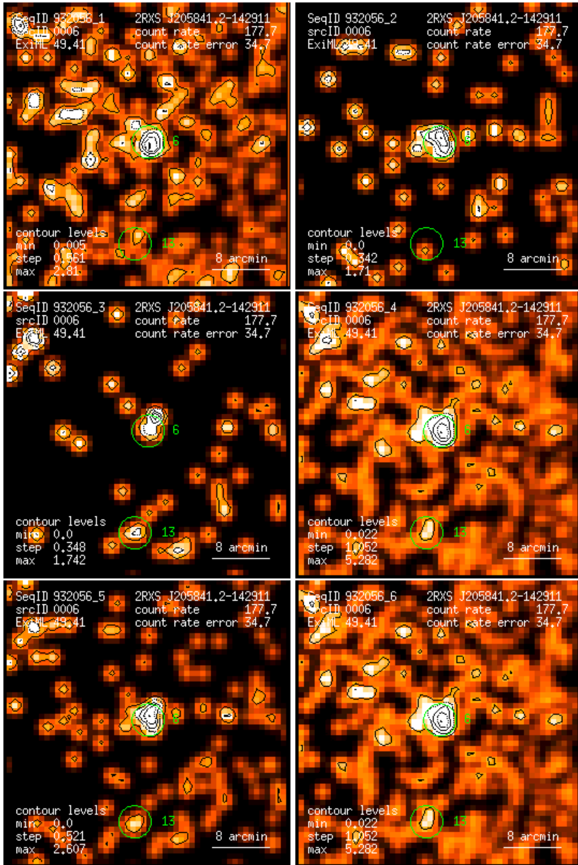
Figure 6: RASS 932056: detection 0006: band rate images, Gaussian filter: (1) PSPC channels 11 – 41, (2) 52 – 90, (3) 91 – 201, (4) 11 – 235, (5) 52 – 201, (6) 11 – 201. Broad band rates in counts/ks. Band rate contour levels in counts/ks/arcmin 2 .
