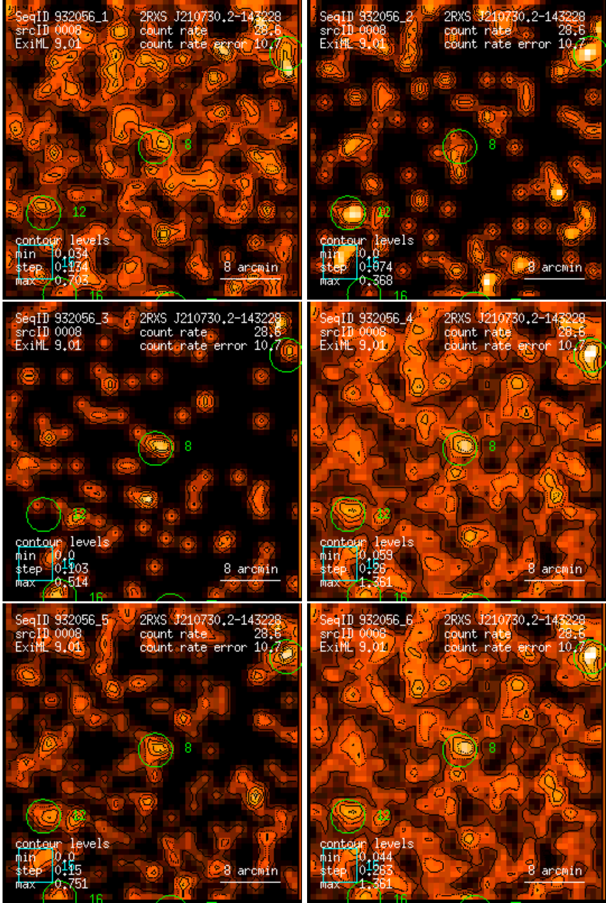
Figure 8: RASS 932056: detection 0008: band rate images, Gaussian filter: (1) PSPC channels 11 – 41, (2) 52 – 90, (3) 91 – 201, (4) 11 – 235, (5) 52 – 201, (6) 11 – 201. Broad band rates in counts/ks. Band rate contour levels in counts/ks/arcmin 2 .
