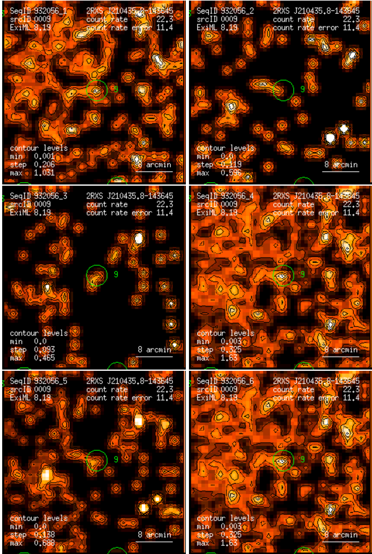
Figure 9: RASS 932056: detection 0009: band rate images, Gaussian filter: (1) PSPC channels 11 – 41, (2) 52 – 90, (3) 91 – 201, (4) 11 – 235, (5) 52 – 201, (6) 11 – 201. Broad band rates in counts/ks. Band rate contour levels in counts/ks/arcmin 2 .
