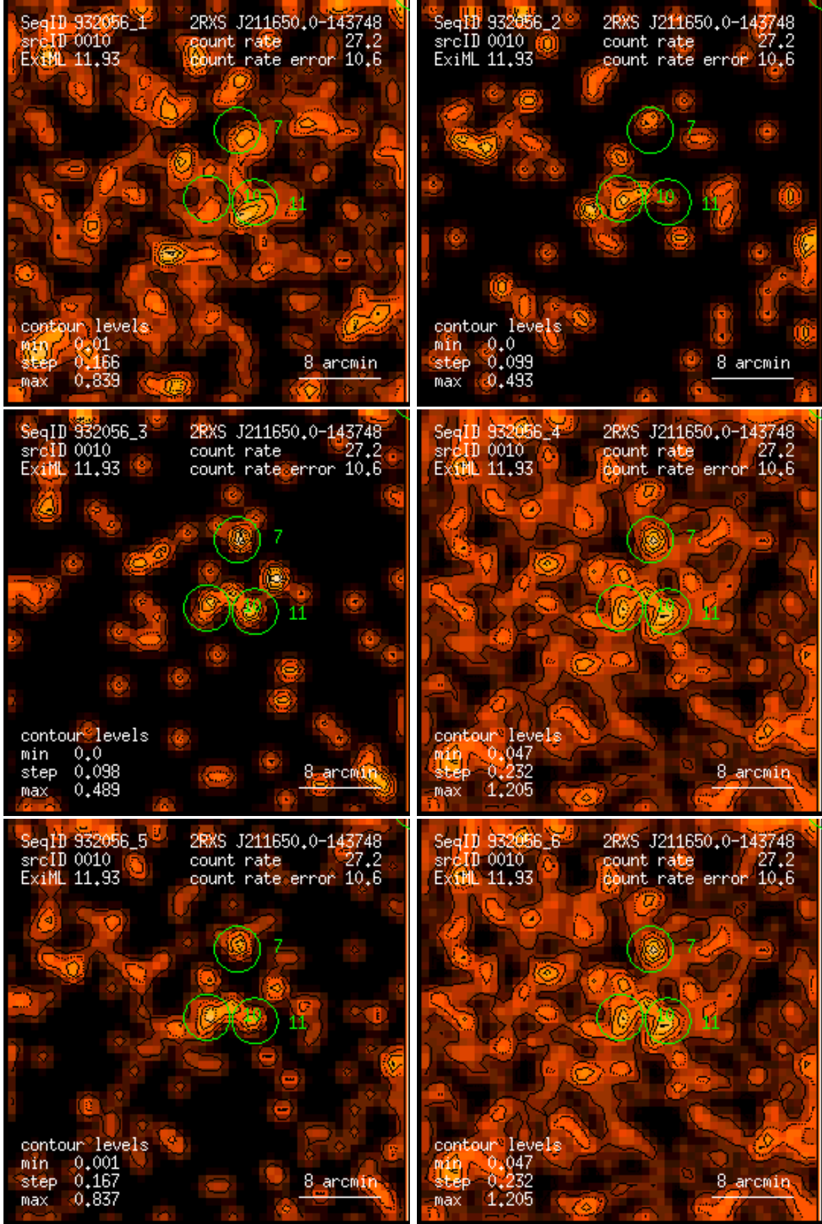
Figure 10: RASS 932056: detection 0010: band rate images, Gaussian filter: (1) PSPC channels 11 – 41, (2) 52 – 90, (3) 91 – 201, (4) 11 – 235, (5) 52 – 201, (6) 11 – 201. Broad band rates in counts/ks. Band rate contour levels in counts/ks/arcmin 2 .
