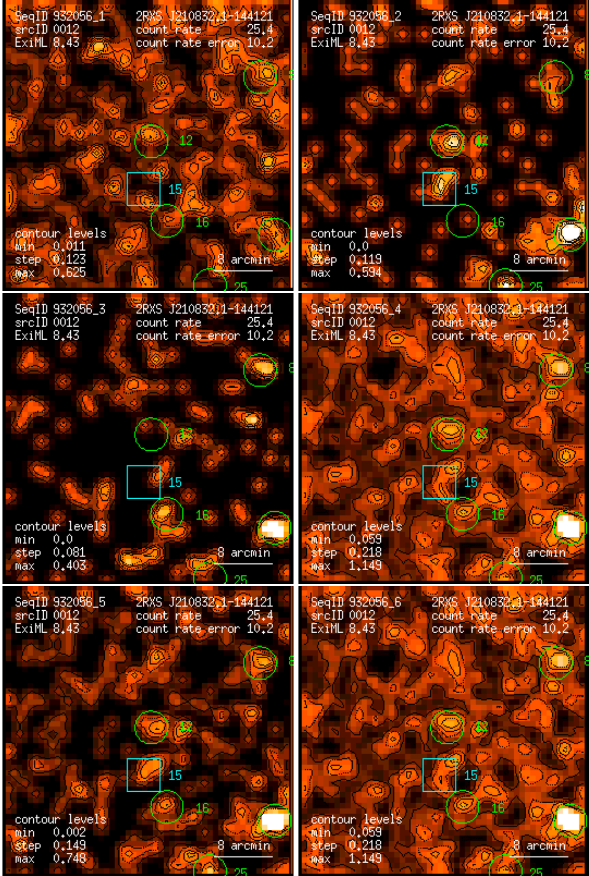
Figure 12: RASS 932056: detection 0012: band rate images, Gaussian filter: (1) PSPC channels 11 – 41, (2) 52 – 90, (3) 91 – 201, (4) 11 – 235, (5) 52 – 201, (6) 11 – 201. Broad band rates in counts/ks. Band rate contour levels in counts/ks/arcmin 2 .
