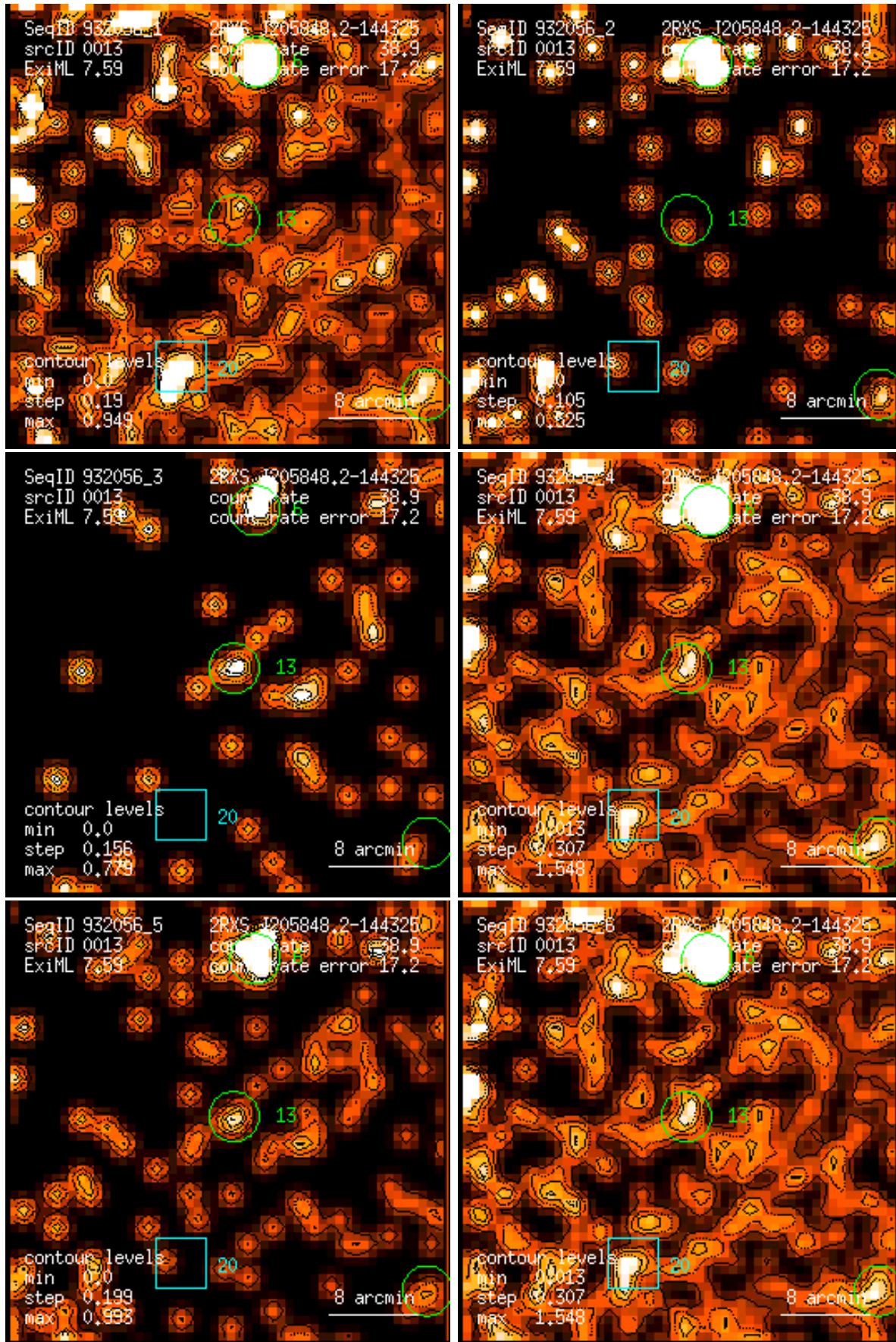
Figure 13: RASS 932056: detection 0013: band rate images, Gaussian filter: (1) PSPC channels 11 – 41, (2) 52 – 90, (3) 91 – 201, (4) 11 – 235, (5) 52 – 201, (6) 11 – 201. Broad band rates in counts/ks. Band rate contour levels in counts/ks/arcmin 2 .
