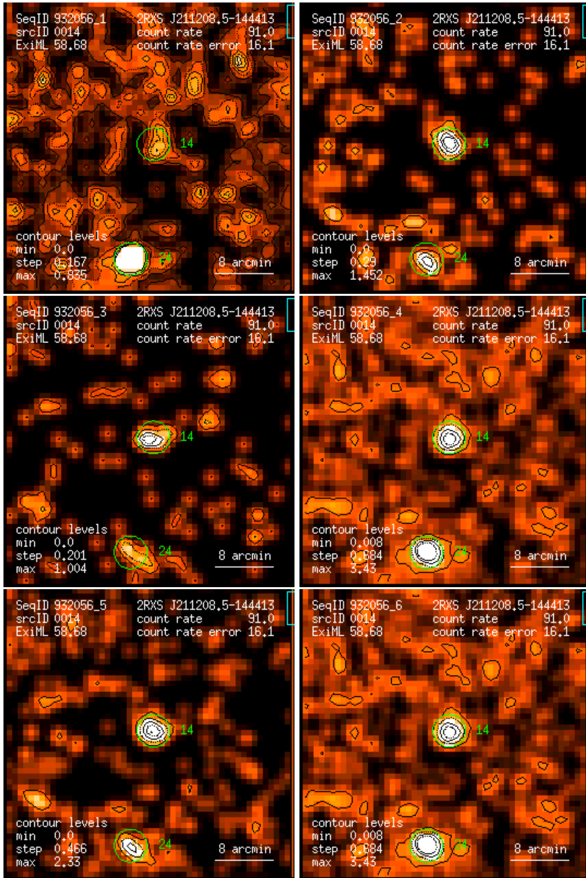
Figure 14: RASS 932056: detection 0014: band rate images, Gaussian filter: (1) PSPC channels 11 – 41, (2) 52 – 90, (3) 91 – 201, (4) 11 – 235, (5) 52 – 201, (6) 11 – 201. Broad band rates in counts/ks. Band rate contour levels in counts/ks/arcmin 2 .
