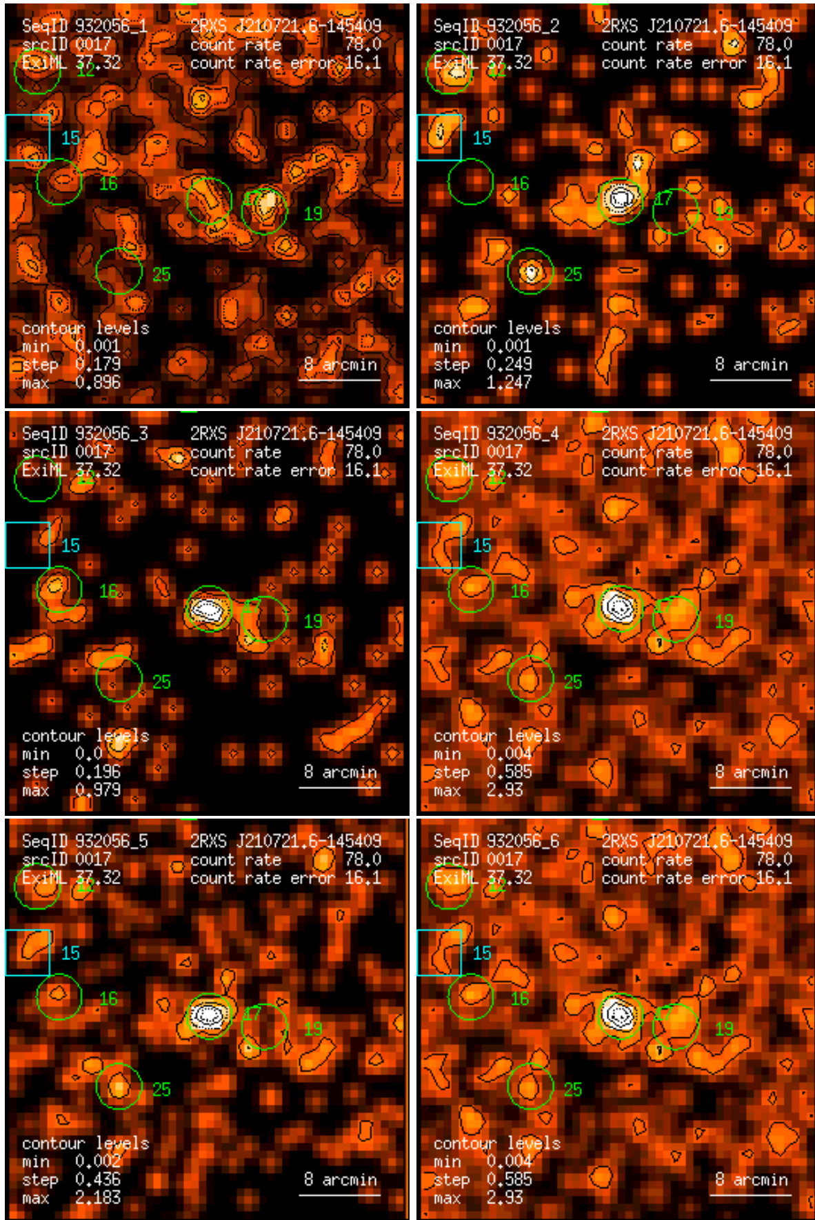
Figure 17: RASS 932056: detection 0017: band rate images, Gaussian filter: (1) PSPC channels 11 – 41, (2) 52 – 90, (3) 91 – 201, (4) 11 – 235, (5) 52 – 201, (6) 11 – 201. Broad band rates in counts/ks. Band rate contour levels in counts/ks/arcmin 2 .
