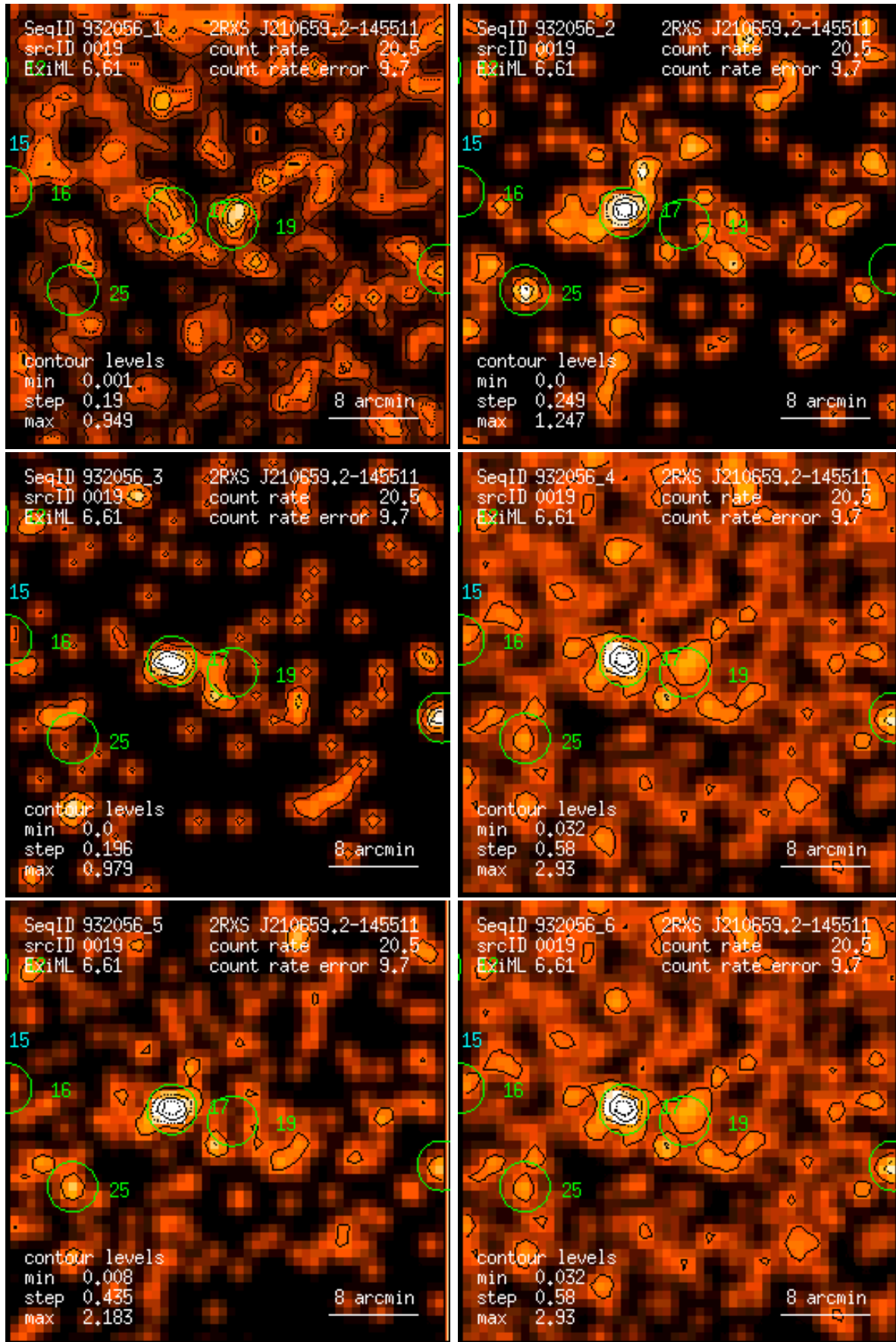
Figure 19: RASS 932056: detection 0019: band rate images, Gaussian filter: (1) PSPC channels 11 – 41, (2) 52 – 90, (3) 91 – 201, (4) 11 – 235, (5) 52 – 201, (6) 11 – 201. Broad band rates in counts/ks. Band rate contour levels in counts/ks/arcmin 2 .
