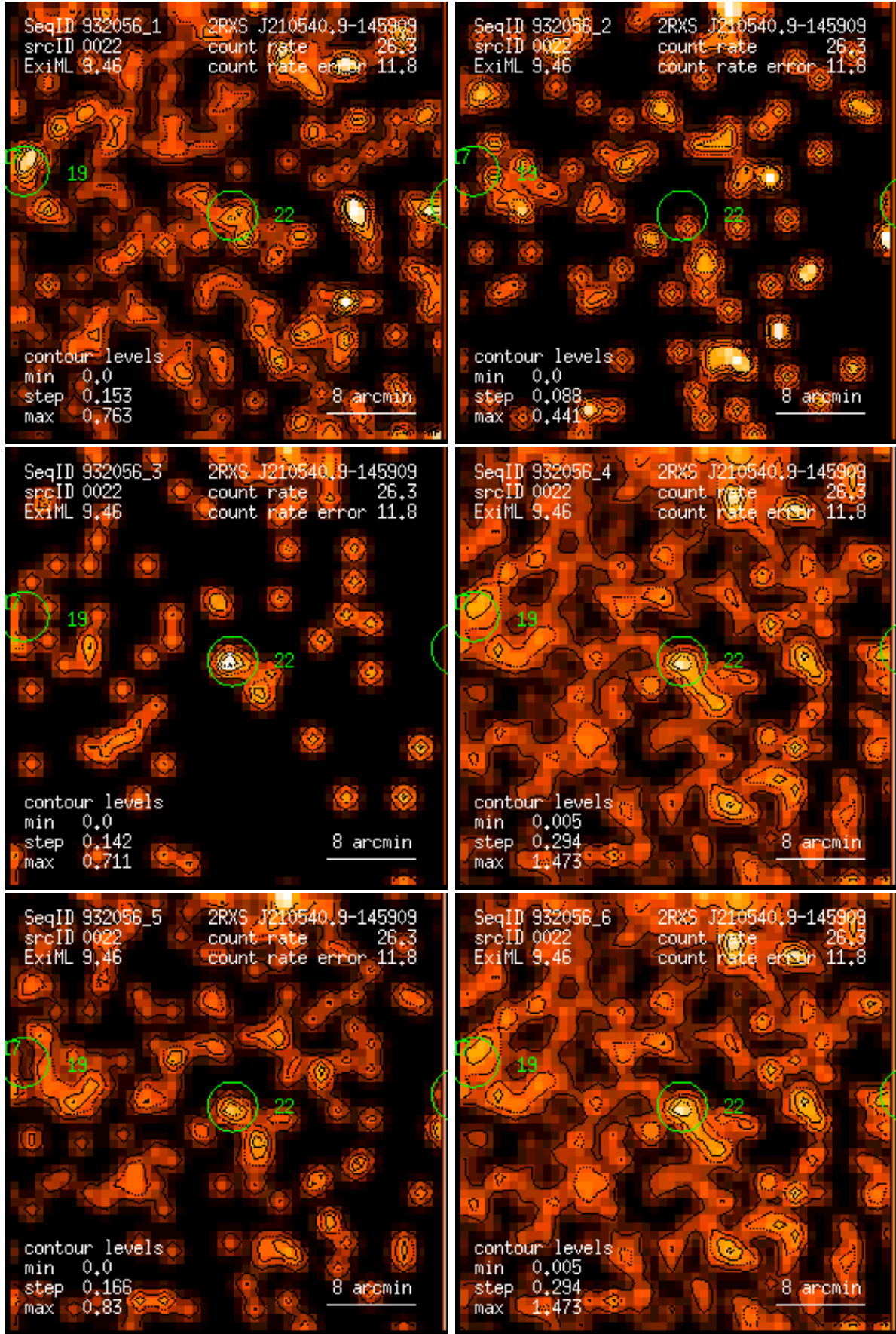
Figure 22: RASS 932056: detection 0022: band rate images, Gaussian filter: (1) PSPC channels 11 – 41, (2) 52 – 90, (3) 91 – 201, (4) 11 – 235, (5) 52 – 201, (6) 11 – 201. Broad band rates in counts/ks. Band rate contour levels in counts/ks/arcmin 2 .
