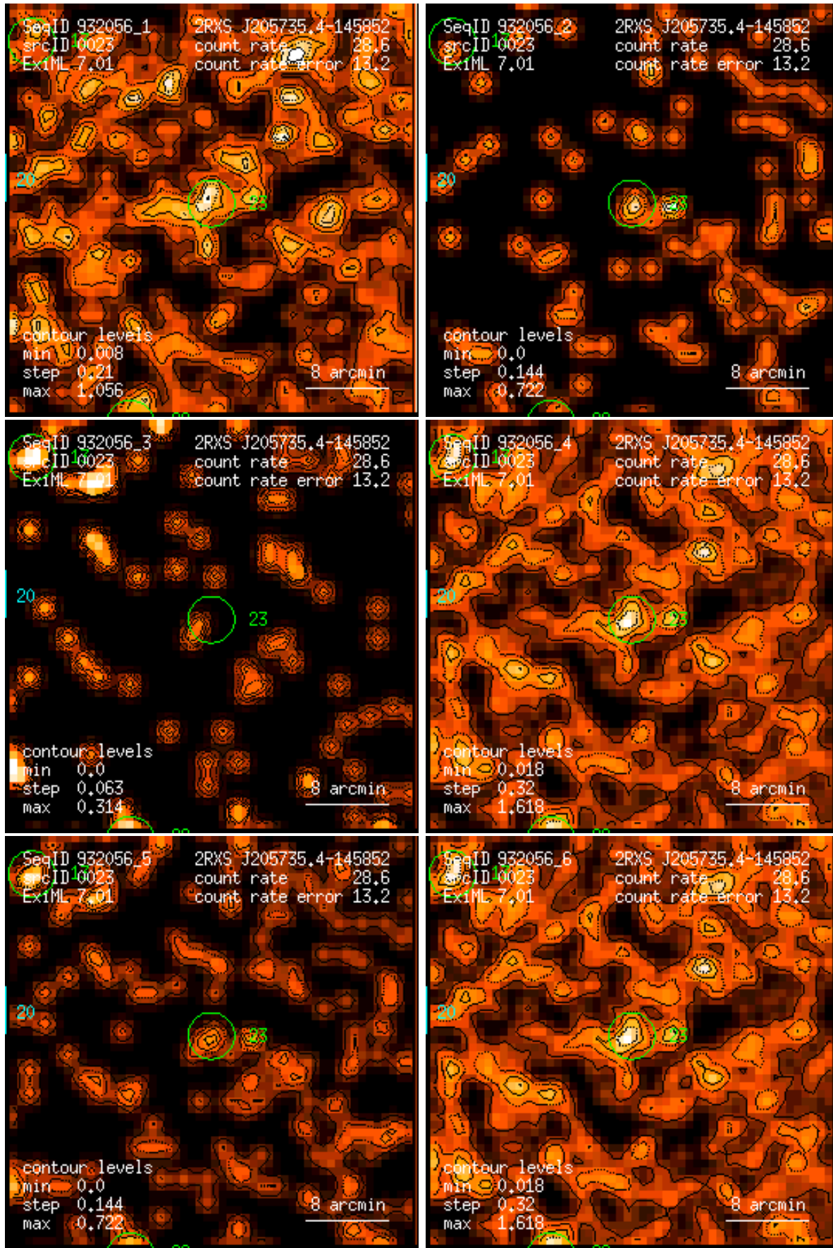
Figure 23: RASS 932056: detection 0023: band rate images, Gaussian filter: (1) PSPC channels 11 – 41, (2) 52 – 90, (3) 91 – 201, (4) 11 – 235, (5) 52 – 201, (6) 11 – 201. Broad band rates in counts/ks. Band rate contour levels in counts/ks/arcmin 2 .
