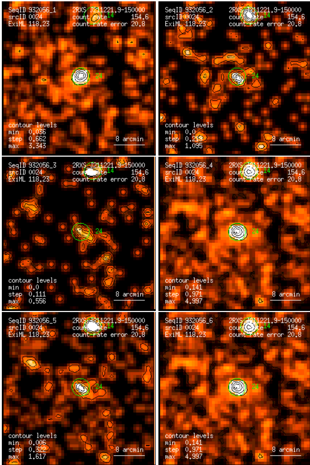
Figure 24: RASS 932056: detection 0024: band rate images, Gaussian filter: (1) PSPC channels 11 – 41, (2) 52 – 90, (3) 91 – 201, (4) 11 – 235, (5) 52 – 201, (6) 11 – 201. Broad band rates in counts/ks. Band rate contour levels in counts/ks/arcmin 2 .
