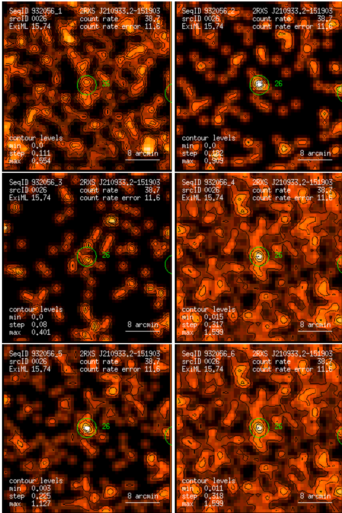
Figure 26: RASS 932056: detection 0026: band rate images, Gaussian filter: (1) PSPC channels 11 – 41, (2) 52 – 90, (3) 91 – 201, (4) 11 – 235, (5) 52 – 201, (6) 11 – 201. Broad band rates in counts/ks. Band rate contour levels in counts/ks/arcmin 2 .
