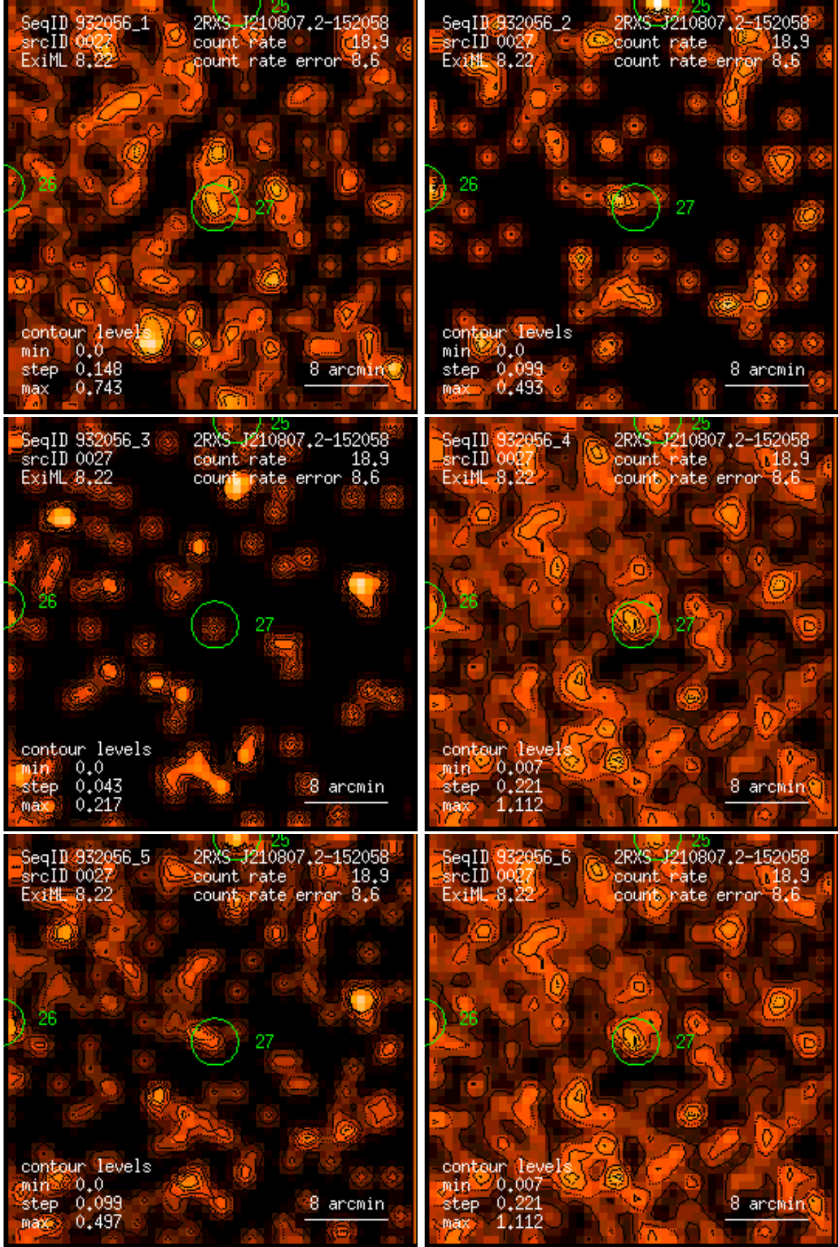
Figure 27: RASS 932056: detection 0027: band rate images, Gaussian filter: (1) PSPC channels 11 – 41, (2) 52 – 90, (3) 91 – 201, (4) 11 – 235, (5) 52 – 201, (6) 11 – 201. Broad band rates in counts/ks. Band rate contour levels in counts/ks/arcmin 2 .
