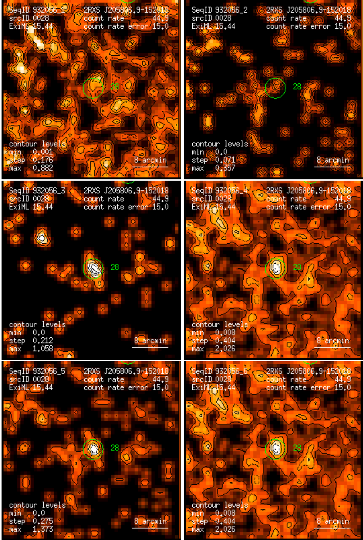
Figure 28: RASS 932056: detection 0028: band rate images, Gaussian filter: (1) PSPC channels 11 – 41, (2) 52 – 90, (3) 91 – 201, (4) 11 – 235, (5) 52 – 201, (6) 11 – 201. Broad band rates in counts/ks. Band rate contour levels in counts/ks/arcmin 2 .
