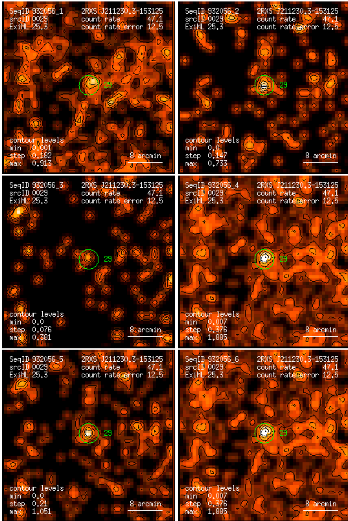
Figure 29: RASS 932056: detection 0029: band rate images, Gaussian filter: (1) PSPC channels 11 – 41, (2) 52 – 90, (3) 91 – 201, (4) 11 – 235, (5) 52 – 201, (6) 11 – 201. Broad band rates in counts/ks. Band rate contour levels in counts/ks/arcmin 2 .
