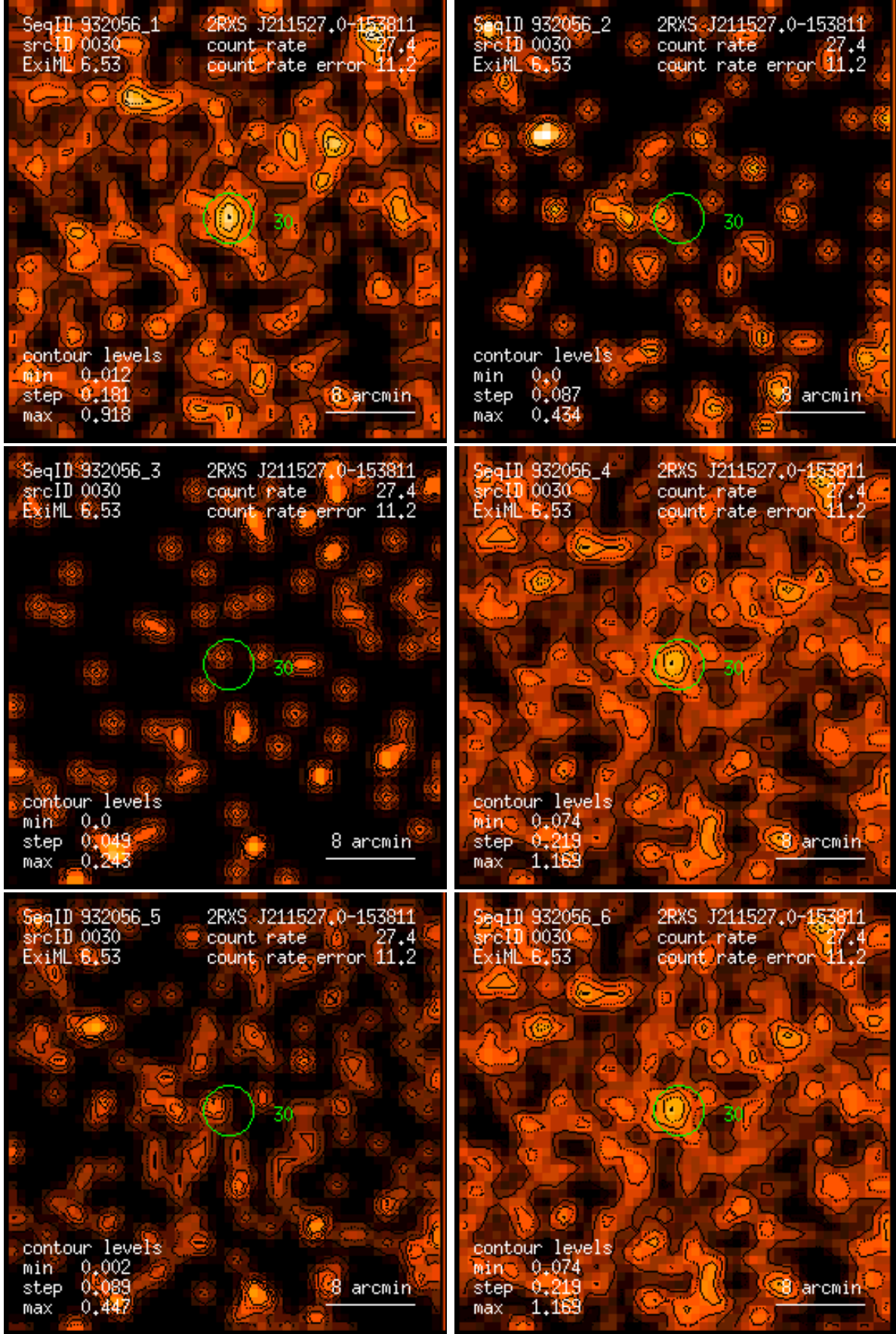
Figure 30: RASS 932056: detection 0030: band rate images, Gaussian filter: (1) PSPC channels 11 – 41, (2) 52 – 90, (3) 91 – 201, (4) 11 – 235, (5) 52 – 201, (6) 11 – 201. Broad band rates in counts/ks. Band rate contour levels in counts/ks/arcmin 2 .
