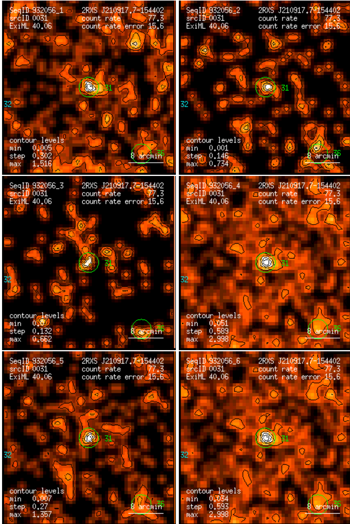
Figure 31: RASS 932056: detection 0031: band rate images, Gaussian filter: (1) PSPC channels 11 – 41, (2) 52 – 90, (3) 91 – 201, (4) 11 – 235, (5) 52 – 201, (6) 11 – 201. Broad band rates in counts/ks. Band rate contour levels in counts/ks/arcmin 2 .
