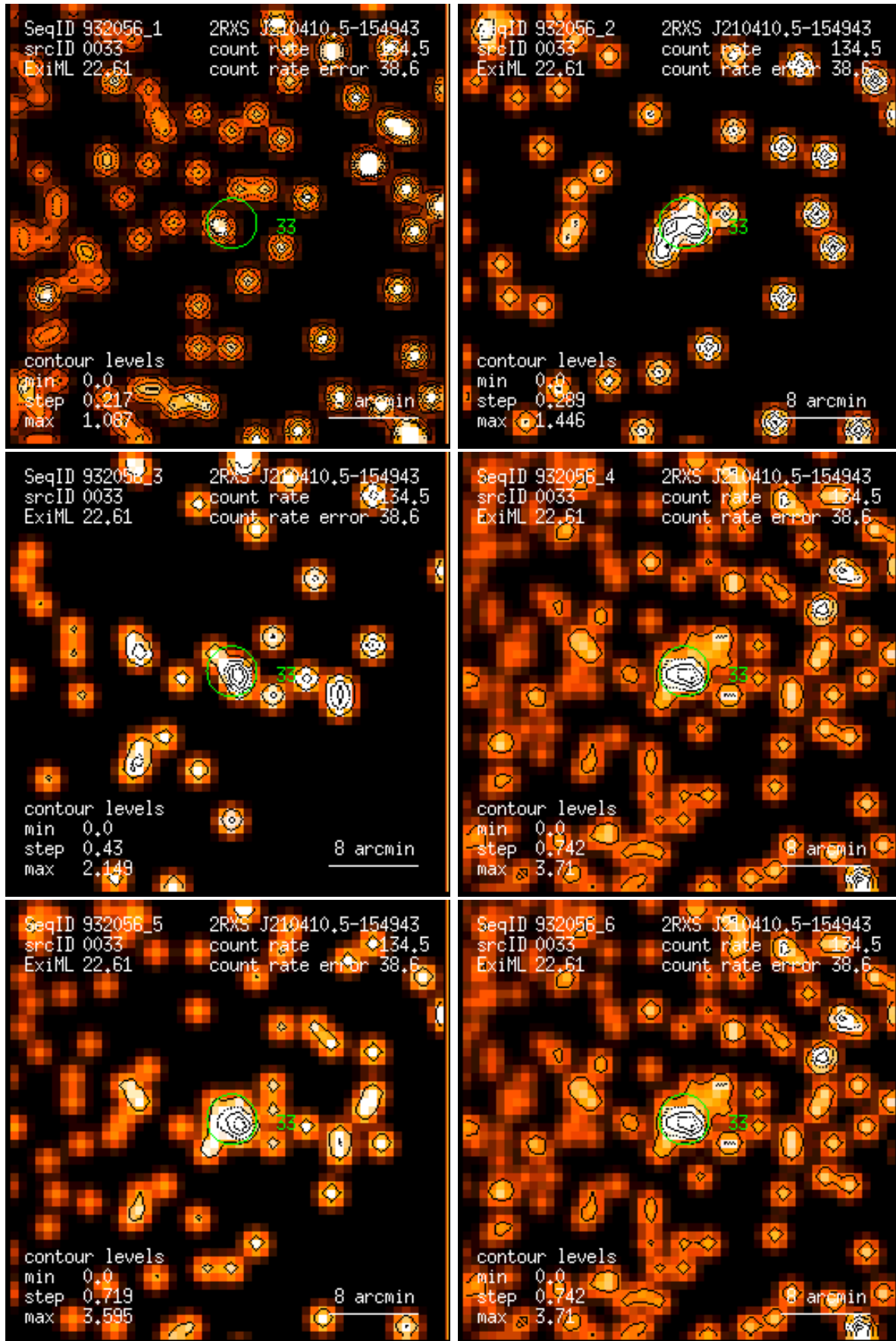
Figure 33: RASS 932056: detection 0033: band rate images, Gaussian filter: (1) PSPC channels 11 – 41, (2) 52 – 90, (3) 91 – 201, (4) 11 – 235, (5) 52 – 201, (6) 11 – 201. Broad band rates in counts/ks. Band rate contour levels in counts/ks/arcmin 2 .
