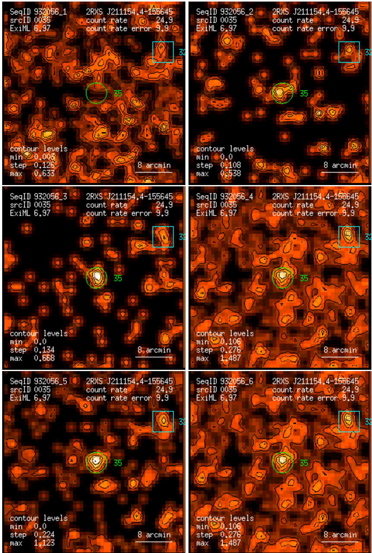
Figure 35: RASS 932056: detection 0035: band rate images, Gaussian filter: (1) PSPC channels 11 – 41, (2) 52 – 90, (3) 91 – 201, (4) 11 – 235, (5) 52 – 201, (6) 11 – 201. Broad band rates in counts/ks. Band rate contour levels in counts/ks/arcmin 2 .
