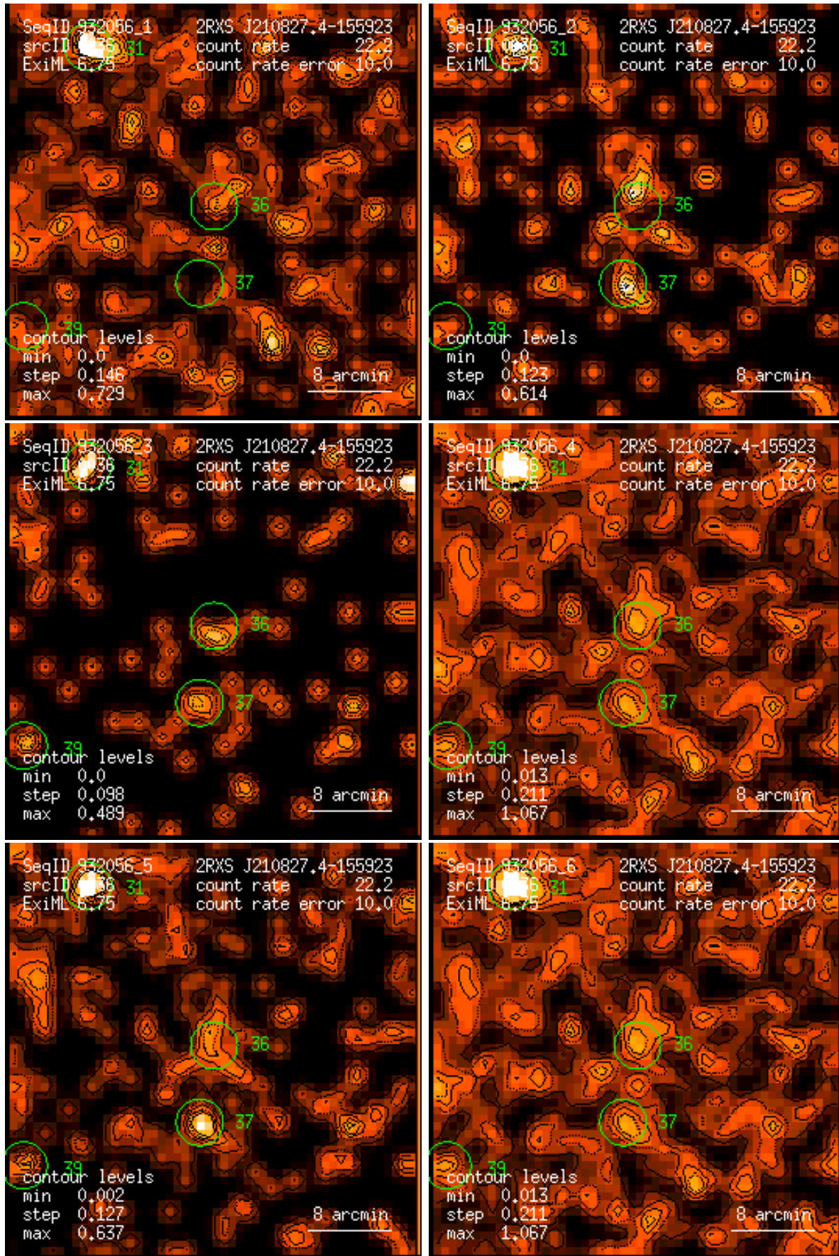
Figure 36: RASS 932056: detection 0036: band rate images, Gaussian filter: (1) PSPC channels 11 – 41, (2) 52 – 90, (3) 91 – 201, (4) 11 – 235, (5) 52 – 201, (6) 11 – 201. Broad band rates in counts/ks. Band rate contour levels in counts/ks/arcmin 2 .
