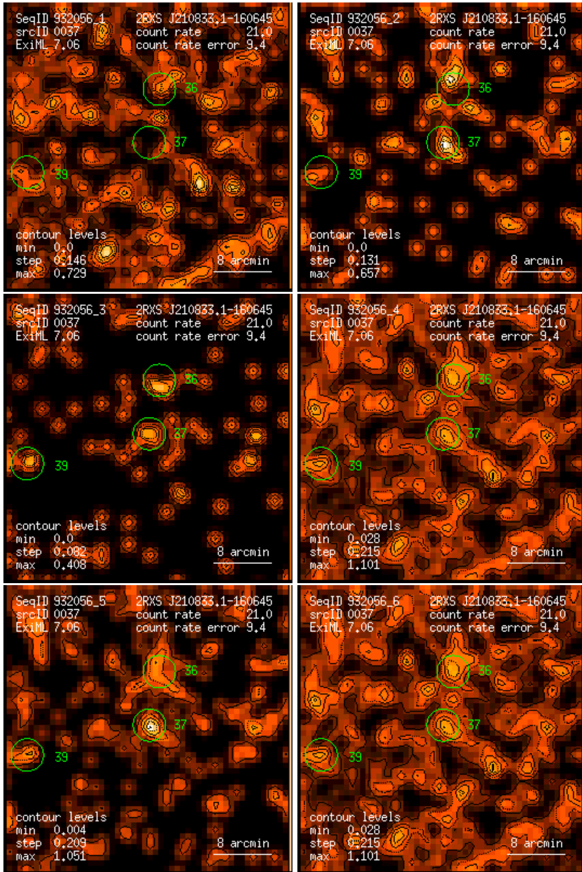
Figure 37: RASS 932056: detection 0037: band rate images, Gaussian filter: (1) PSPC channels 11 – 41, (2) 52 – 90, (3) 91 – 201, (4) 11 – 235, (5) 52 – 201, (6) 11 – 201. Broad band rates in counts/ks. Band rate contour levels in counts/ks/arcmin 2 .
