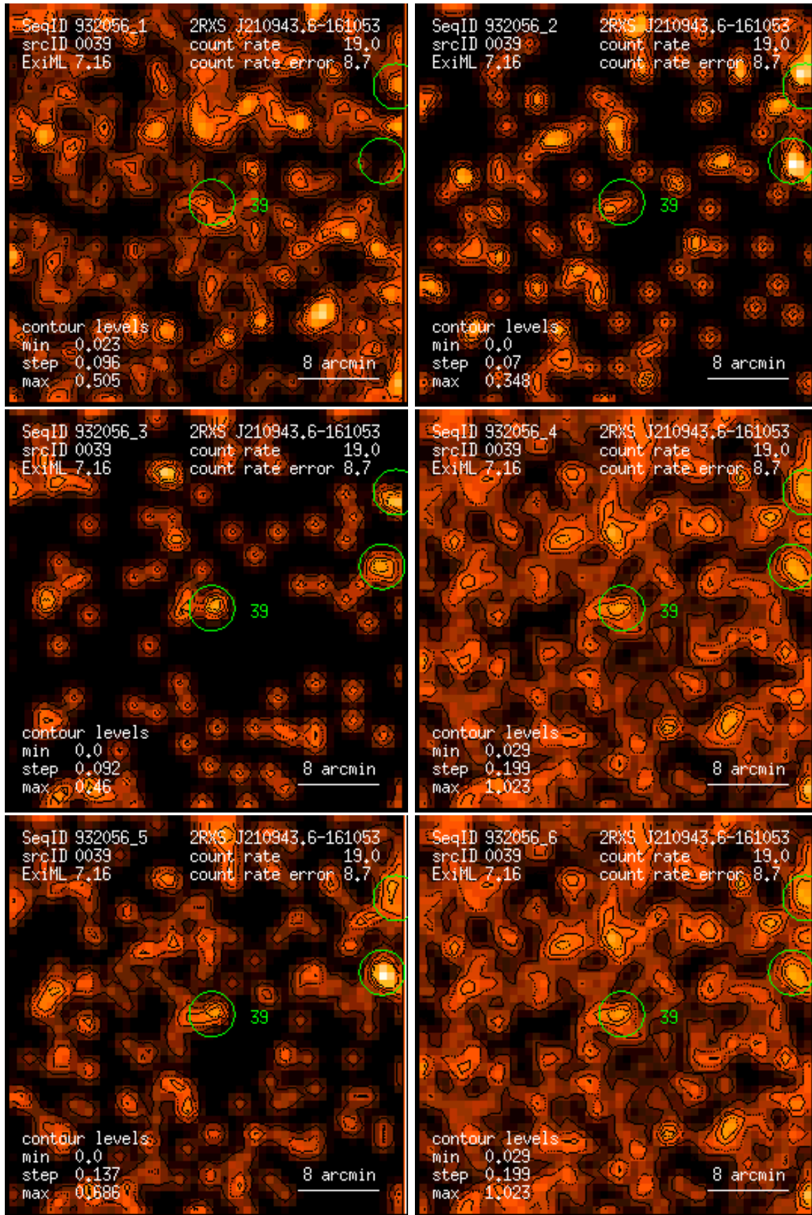
Figure 39: RASS 932056: detection 0039: band rate images, Gaussian filter: (1) PSPC channels 11 – 41, (2) 52 – 90, (3) 91 – 201, (4) 11 – 235, (5) 52 – 201, (6) 11 – 201. Broad band rates in counts/ks. Band rate contour levels in counts/ks/arcmin 2 .
