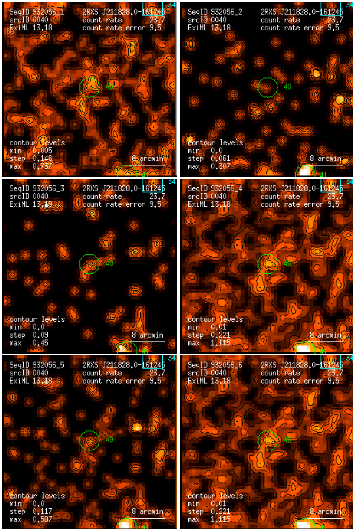
Figure 40: RASS 932056: detection 0040: band rate images, Gaussian filter: (1) PSPC channels 11 – 41, (2) 52 – 90, (3) 91 – 201, (4) 11 – 235, (5) 52 – 201, (6) 11 – 201. Broad band rates in counts/ks. Band rate contour levels in counts/ks/arcmin 2 .
