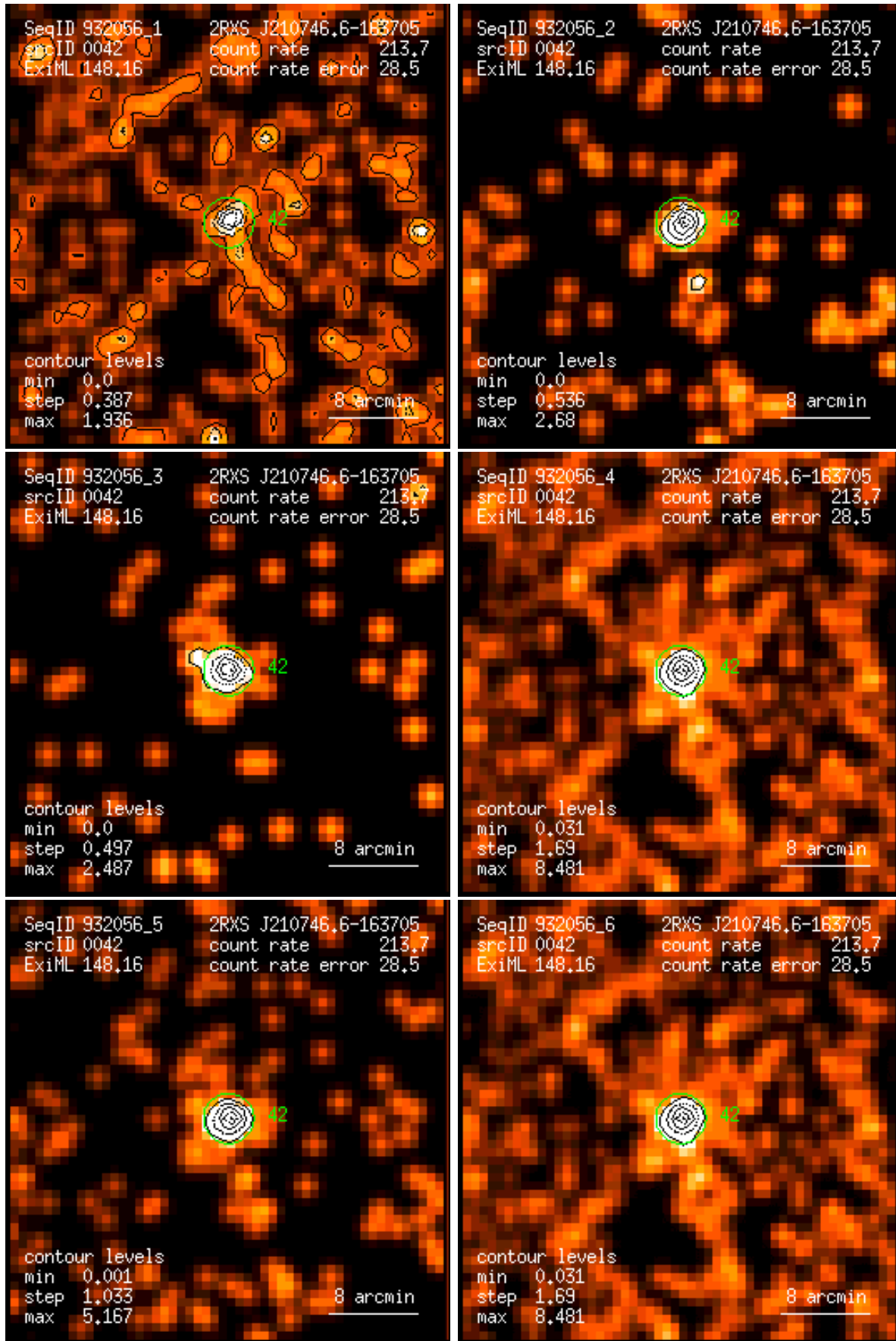
Figure 42: RASS 932056: detection 0042: band rate images, Gaussian filter: (1) PSPC channels 11 – 41, (2) 52 – 90, (3) 91 – 201, (4) 11 – 235, (5) 52 – 201, (6) 11 – 201. Broad band rates in counts/ks. Band rate contour levels in counts/ks/arcmin 2 .
