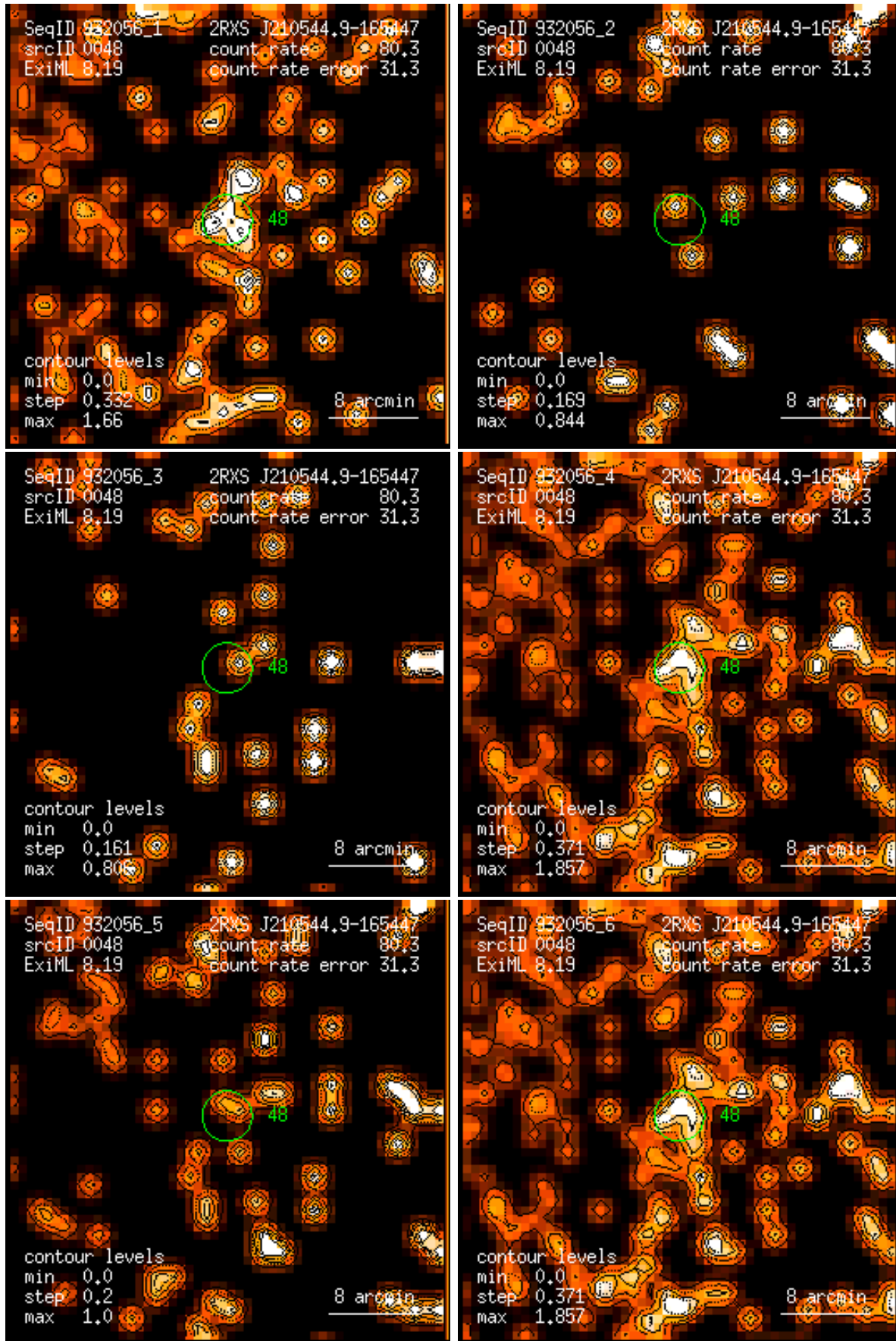
Figure 48: RASS 932056: detection 0048: band rate images, Gaussian filter: (1) PSPC channels 11 – 41, (2) 52 – 90, (3) 91 – 201, (4) 11 – 235, (5) 52 – 201, (6) 11 – 201. Broad band rates in counts/ks. Band rate contour levels in counts/ks/arcmin 2 .
