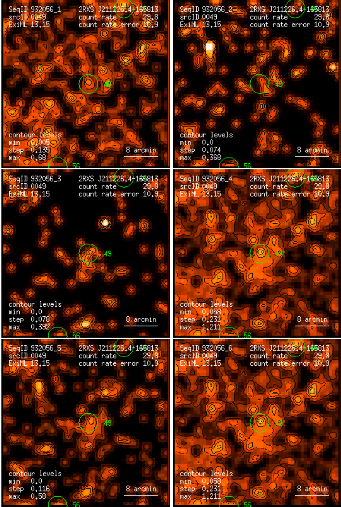
Figure 49: RASS 932056: detection 0049: band rate images, Gaussian filter: (1) PSPC channels 11 – 41, (2) 52 – 90, (3) 91 – 201, (4) 11 – 235, (5) 52 – 201, (6) 11 – 201. Broad band rates in counts/ks. Band rate contour levels in counts/ks/arcmin 2 .
