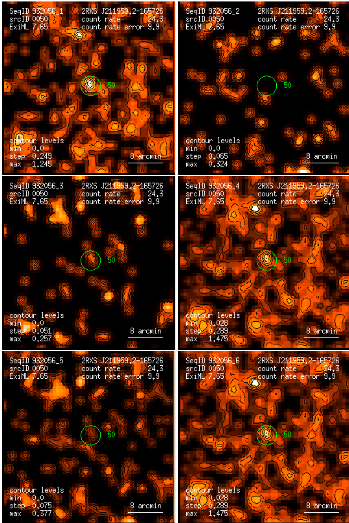
Figure 50: RASS 932056: detection 0050: band rate images, Gaussian filter: (1) PSPC channels 11 – 41, (2) 52 – 90, (3) 91 – 201, (4) 11 – 235, (5) 52 – 201, (6) 11 – 201. Broad band rates in counts/ks. Band rate contour levels in counts/ks/arcmin 2 .
