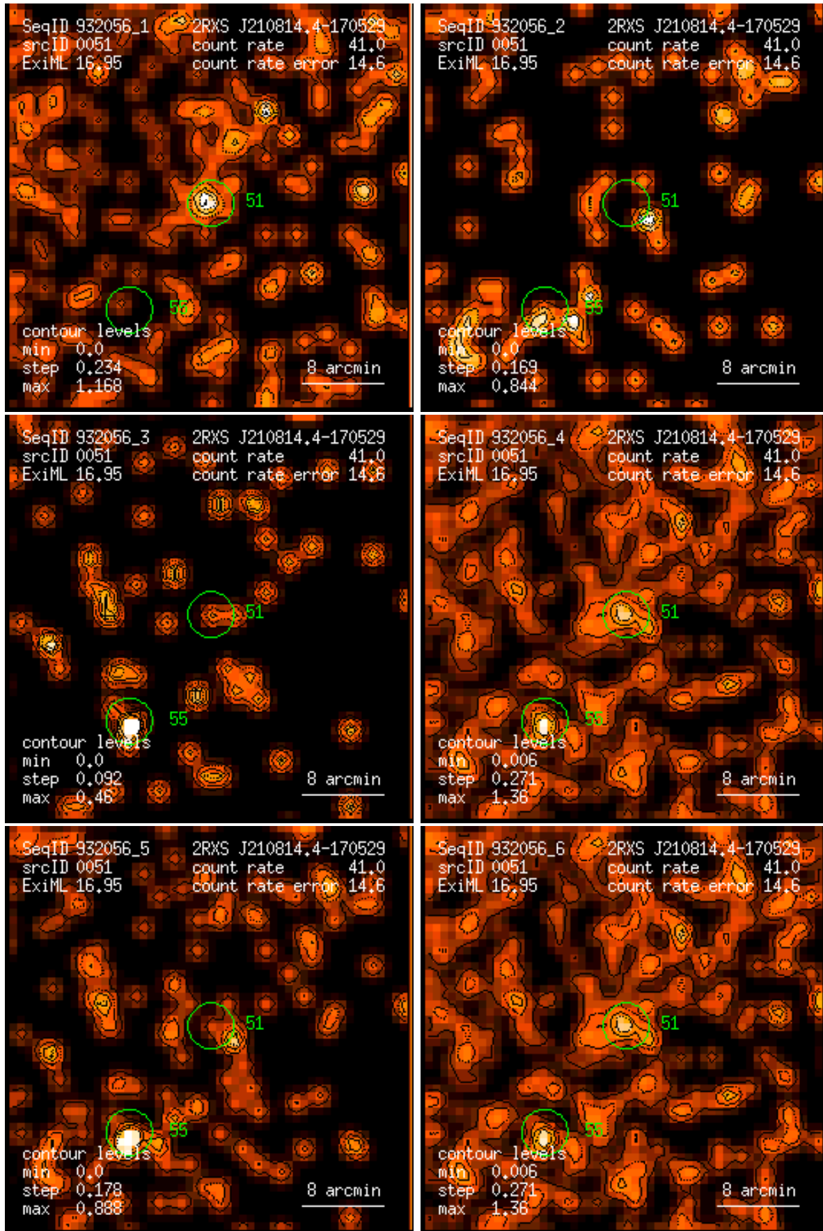
Figure 51: RASS 932056: detection 0051: band rate images, Gaussian filter: (1) PSPC channels 11 – 41, (2) 52 – 90, (3) 91 – 201, (4) 11 – 235, (5) 52 – 201, (6) 11 – 201. Broad band rates in counts/ks. Band rate contour levels in counts/ks/arcmin 2 .
