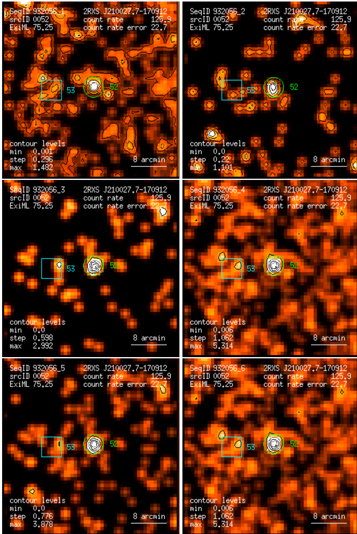
Figure 52: RASS 932056: detection 0052: band rate images, Gaussian filter: (1) PSPC channels 11 – 41, (2) 52 – 90, (3) 91 – 201, (4) 11 – 235, (5) 52 – 201, (6) 11 – 201. Broad band rates in counts/ks. Band rate contour levels in counts/ks/arcmin 2 .
