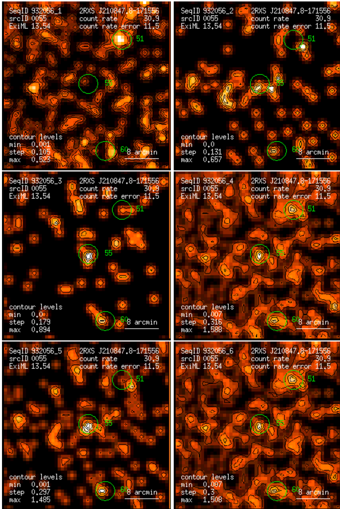
Figure 55: RASS 932056: detection 0055: band rate images, Gaussian filter: (1) PSPC channels 11 – 41, (2) 52 – 90, (3) 91 – 201, (4) 11 – 235, (5) 52 – 201, (6) 11 – 201. Broad band rates in counts/ks. Band rate contour levels in counts/ks/arcmin 2 .
